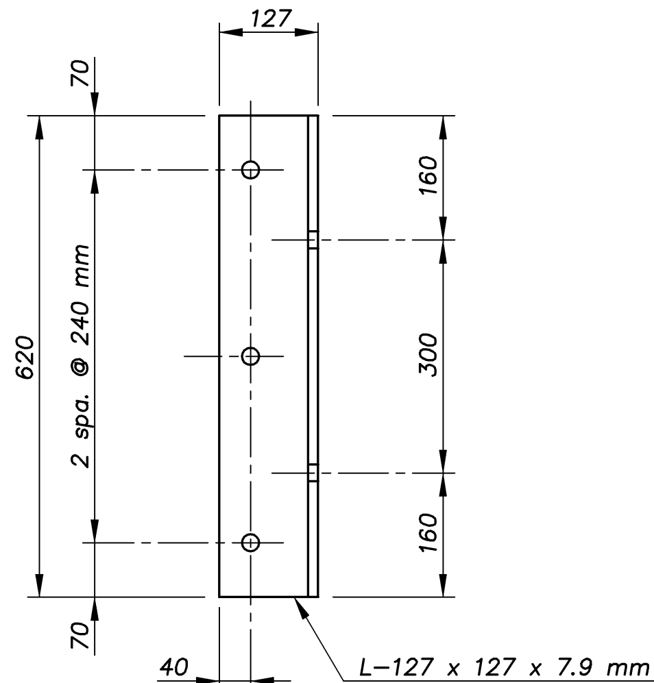
BRACKET
