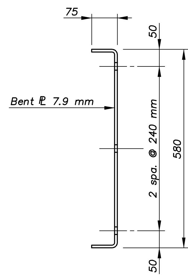
BENT PLATE
