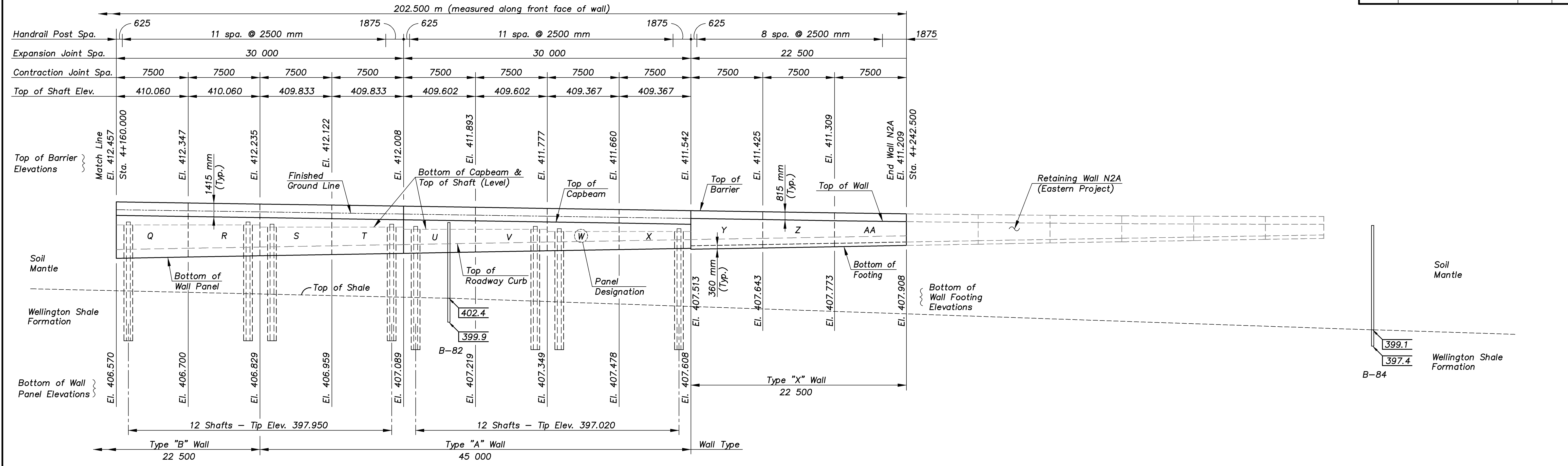
ELEVATION ALONG FRONT FACE OF WALL
