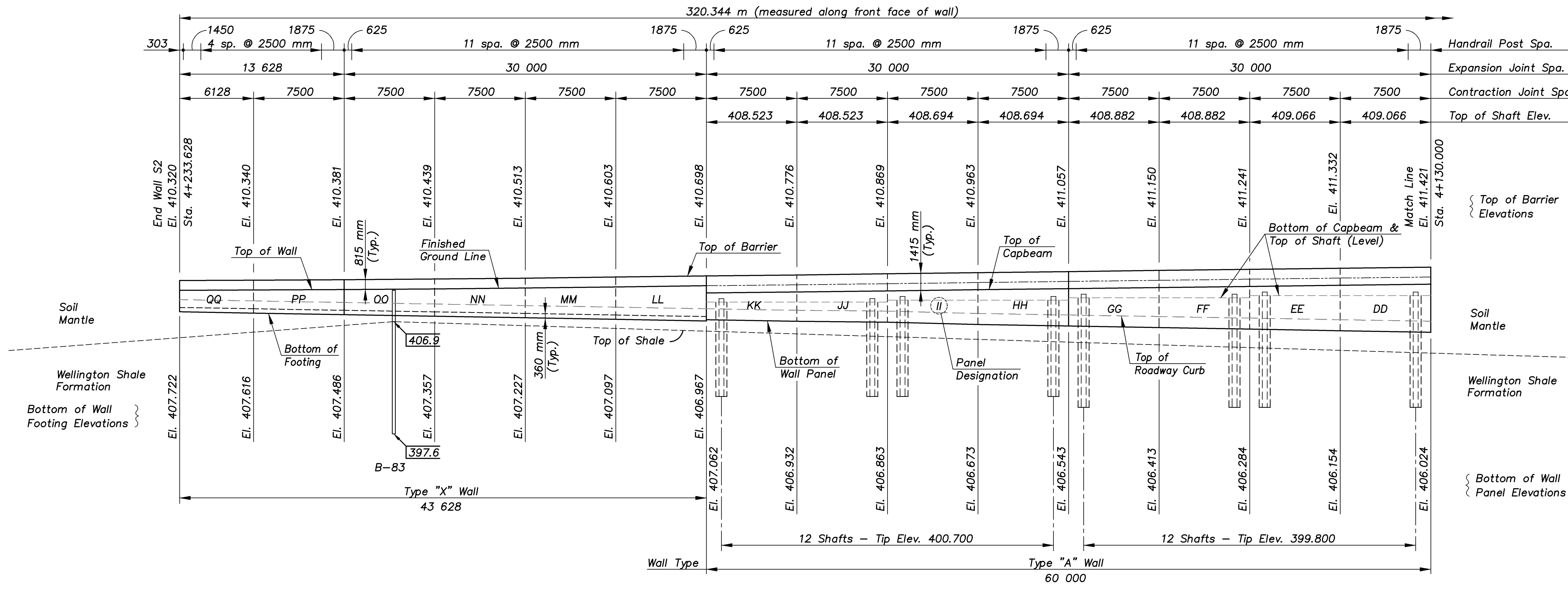
ELEVATION ALONG FRONT FACE OF WALL
