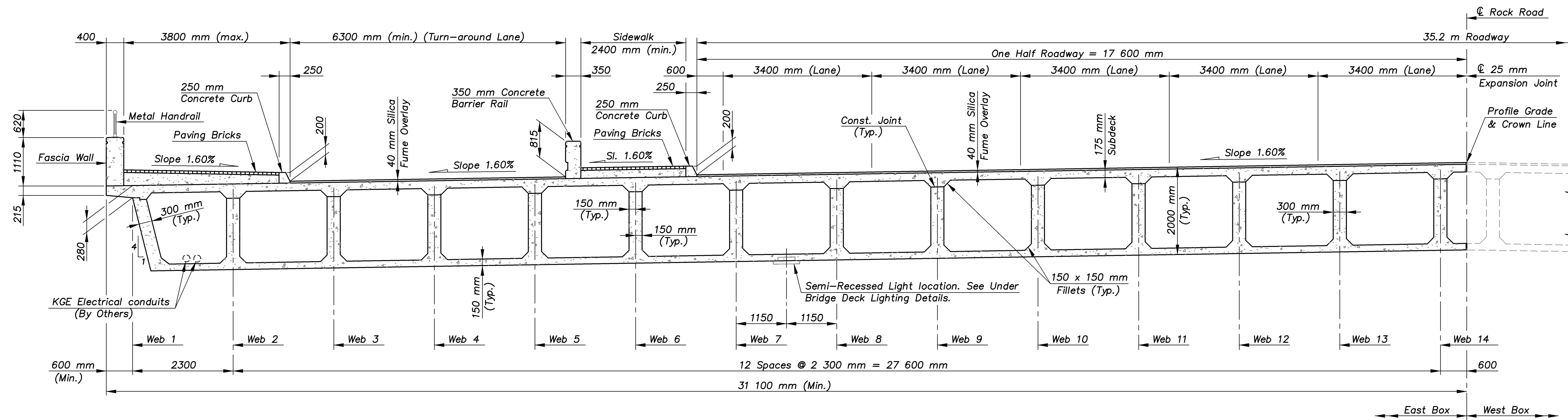
TYPICAL SECTION NORTHBOUND ROCK ROAD OVER KELLOGG (Looking Ahead Station near Mid-Span)
