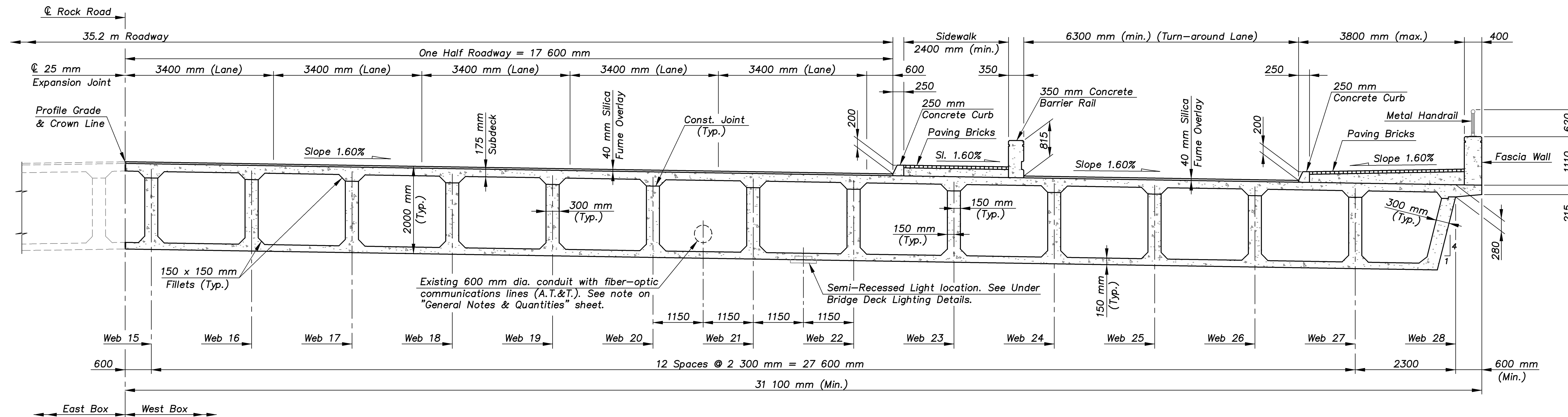
TYPICAL SECTION SOUTHBOUND ROCK ROAD OVER KELLOGG (Looking Ahead Station near Mid-Span)
