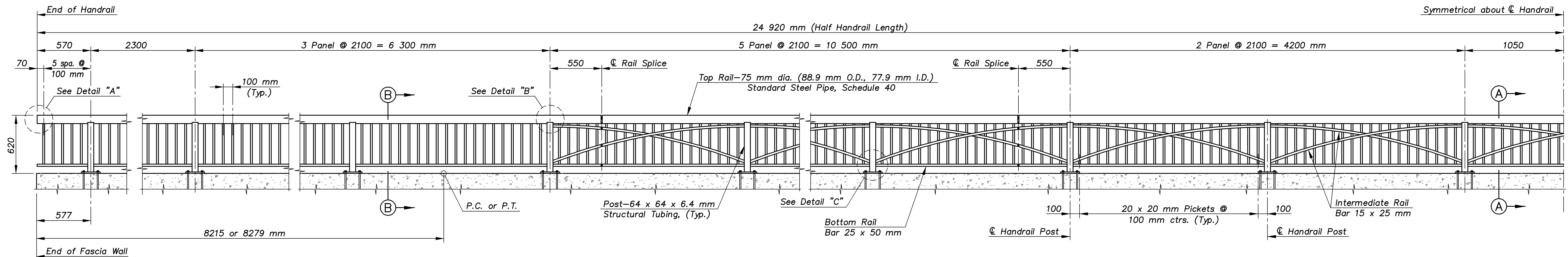
DEVELOPED TYPICAL ELEVATION OF HANDRAIL
