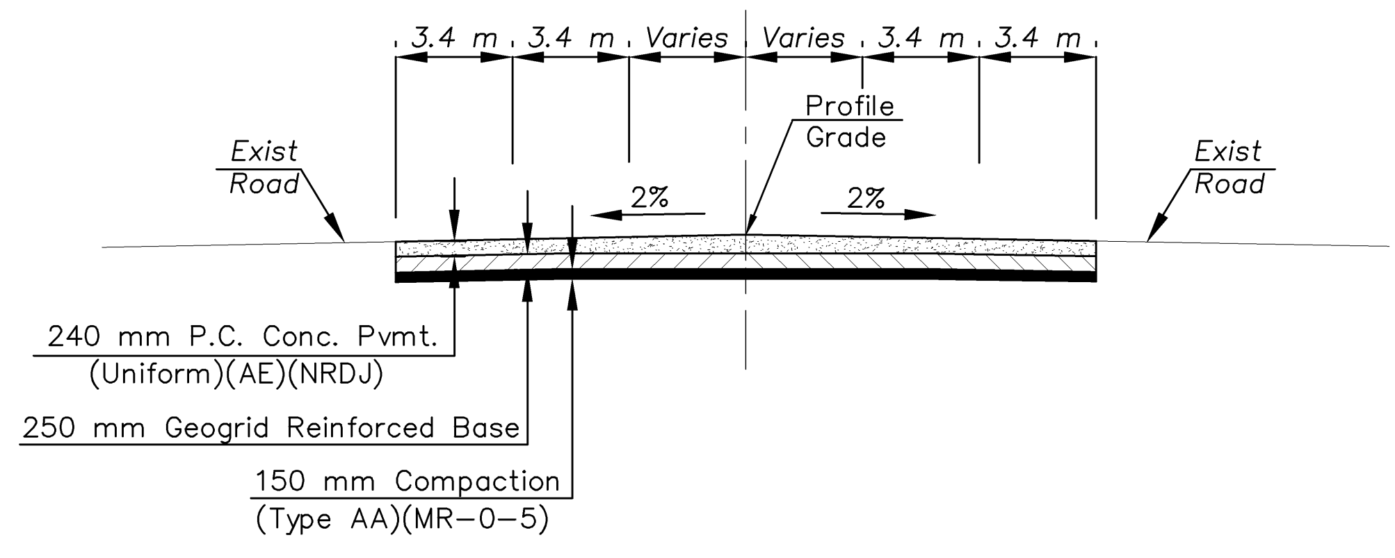
TYPICAL SECTION
