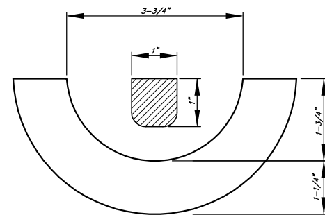
SECTION VIEW
