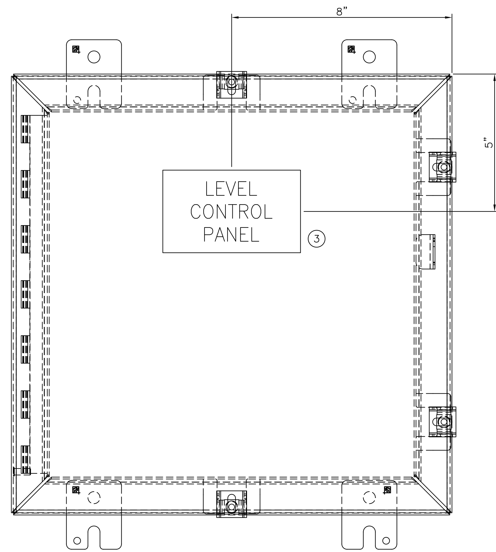
1 LEVEL CONTROL PANEL EXTERIOR LAYOUT SCALE: 1/2" = 1"
