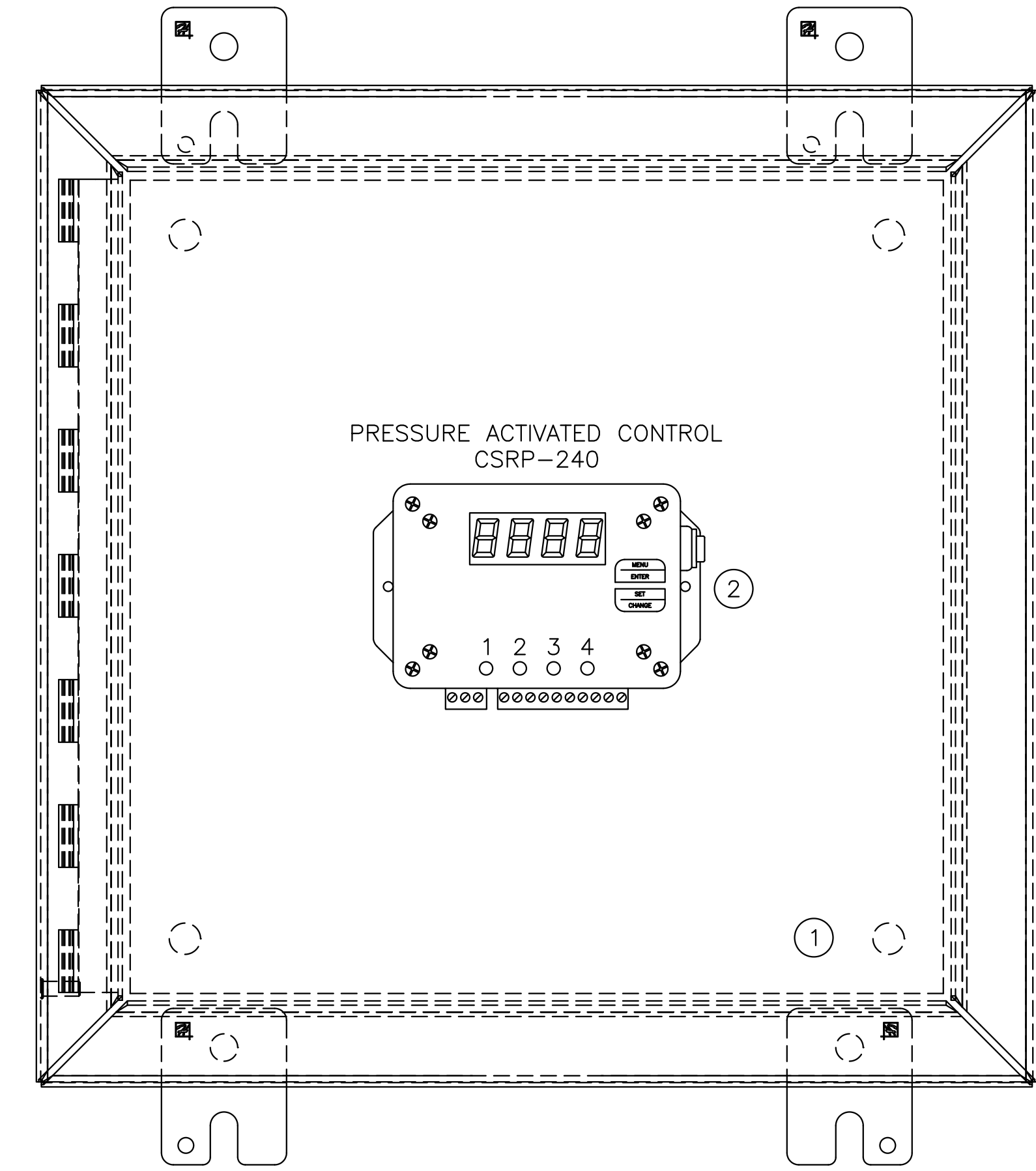
2 LEVEL CONTROL PANEL INTERIOR LAYOUT SCALE: 1/2" = 1"
