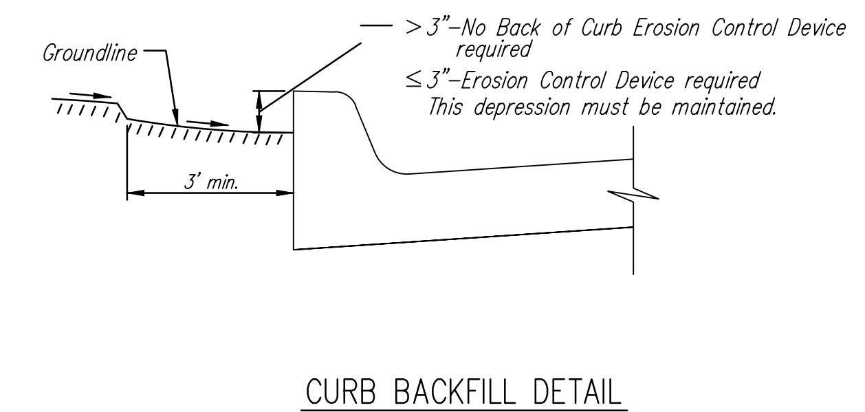
CURB BACKFILL DETAIL
