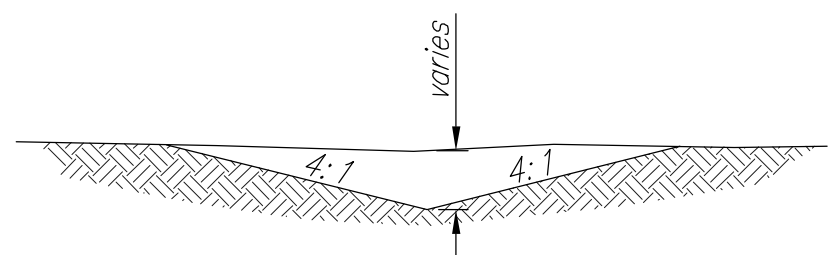
V BOTTOM DITCH DETAIL
