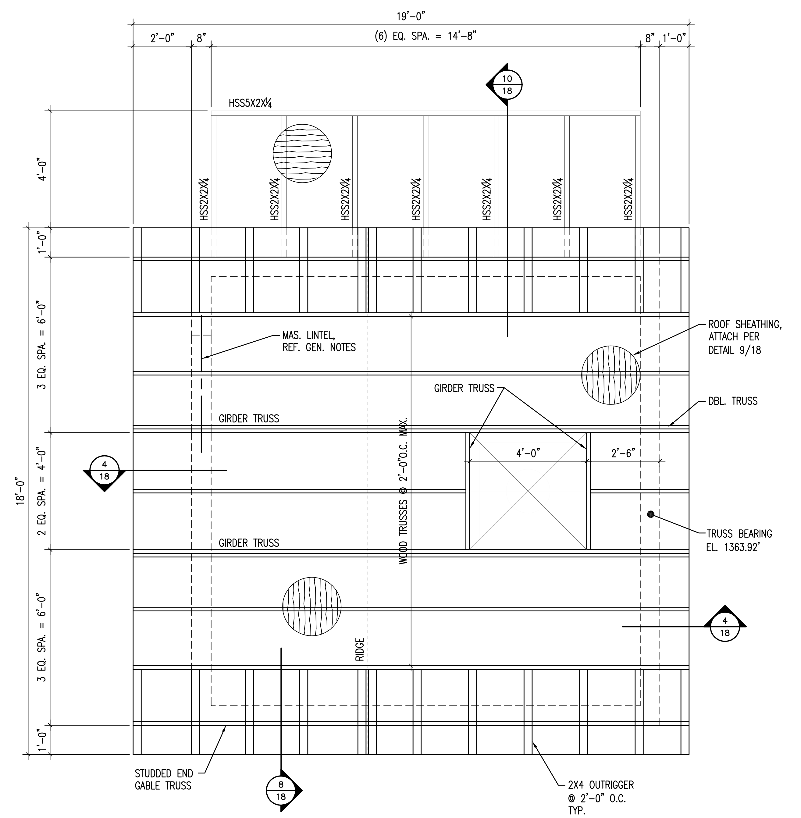
2 ROOF FRAMING PLAN 1/2"=1'-0"
