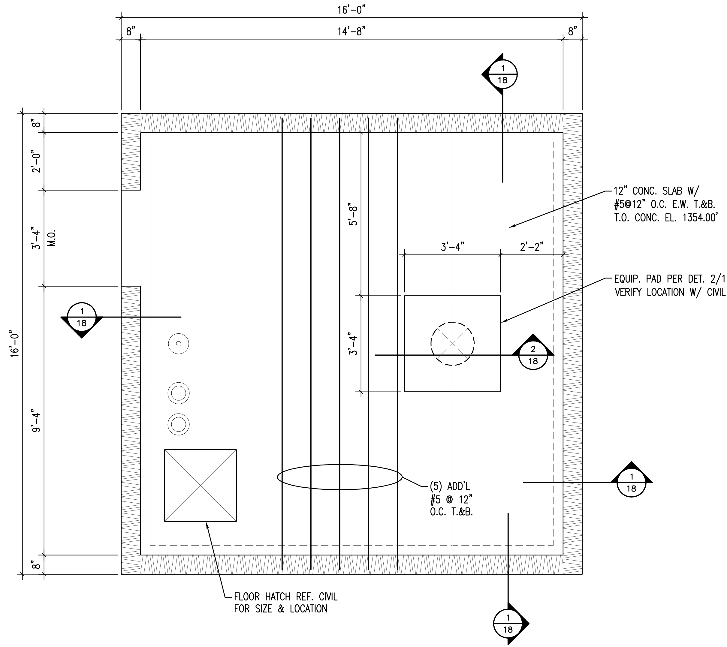
1 MAIN LEVEL PLAN 1/2"=1'-0"
