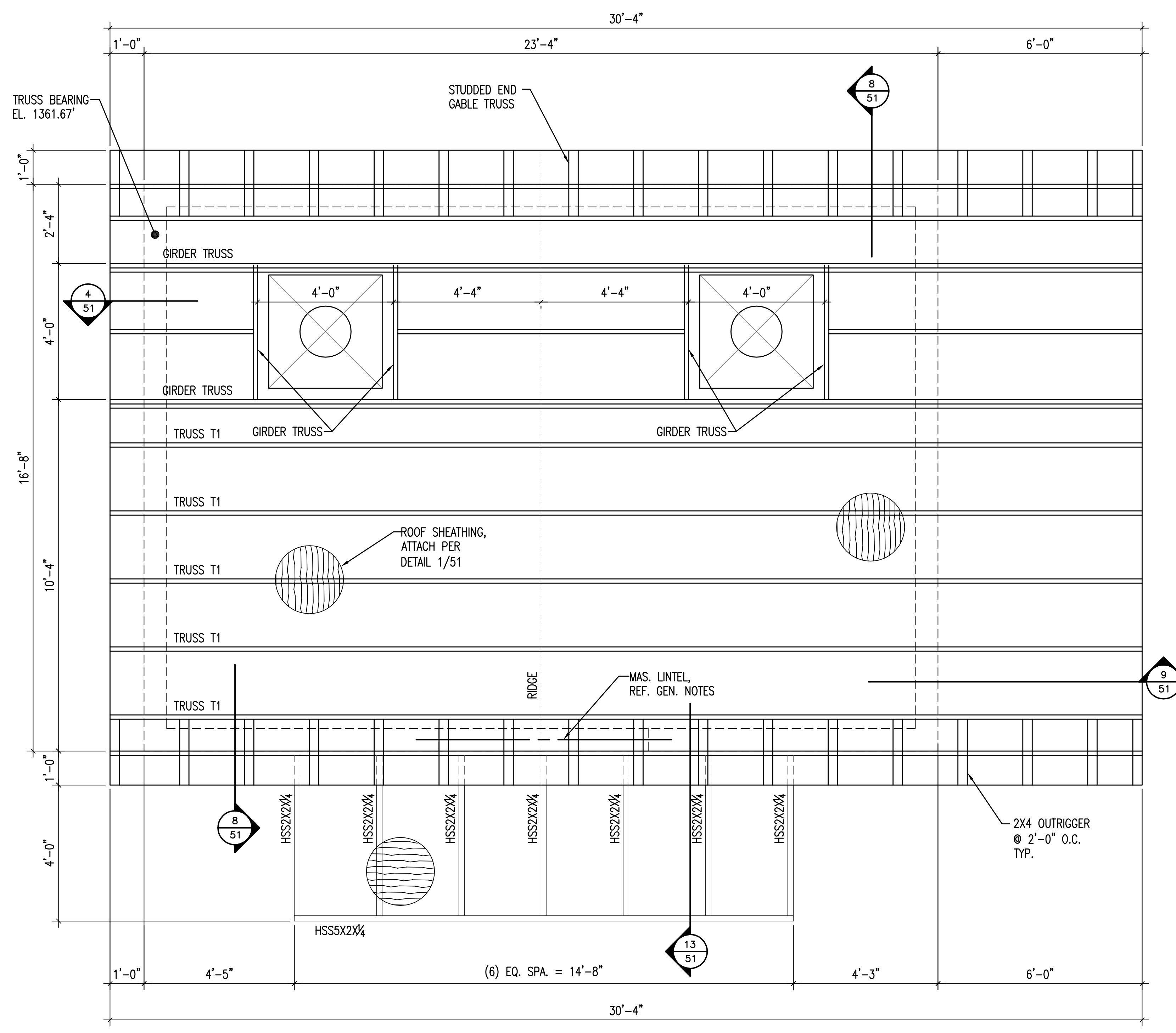
2 ROOF FRAMING PLAN 49 1/2"=1'-0" N W E S
