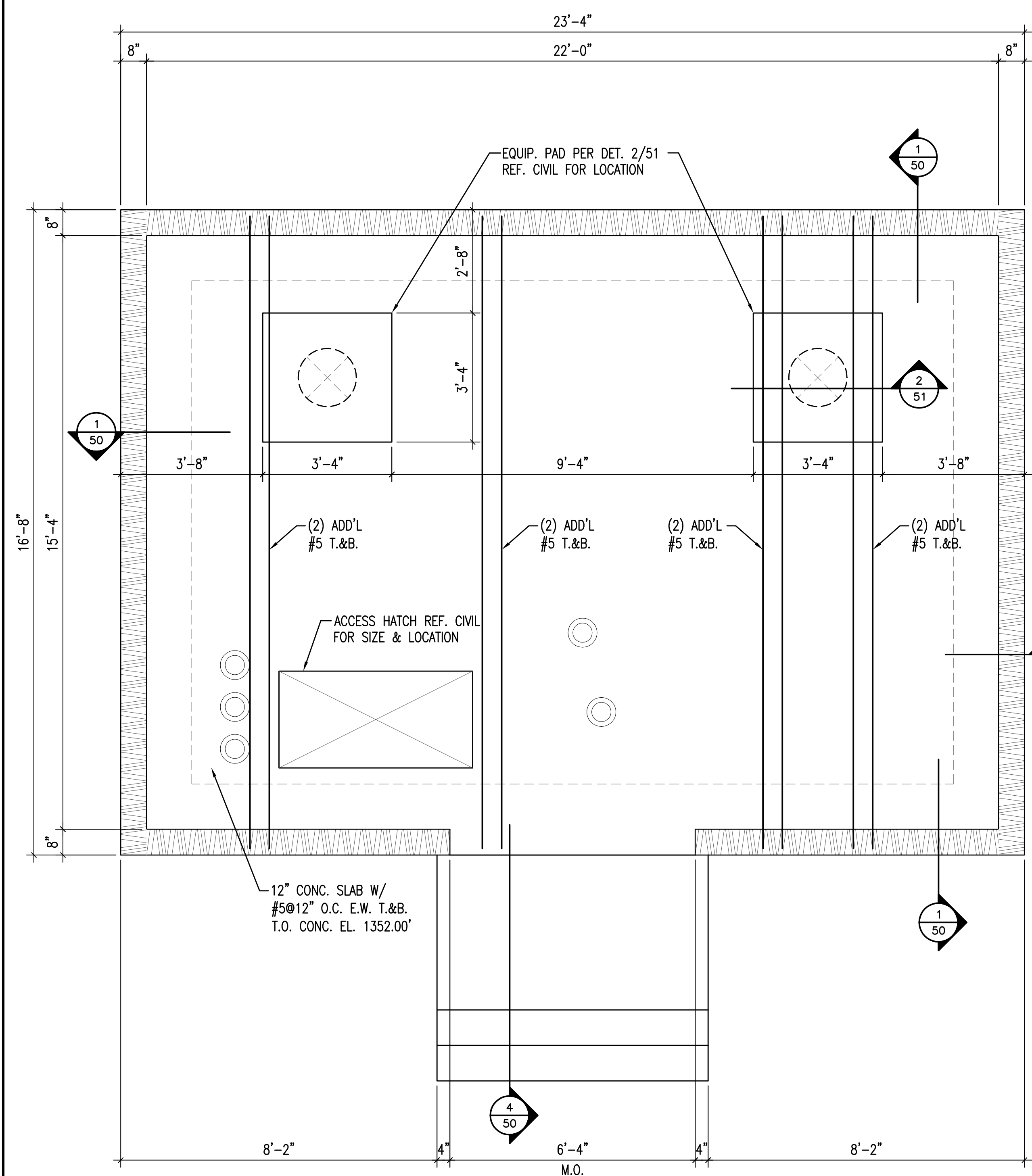
1 MAIN LEVEL PLAN 49 1/2"=1'-0" N W E S
