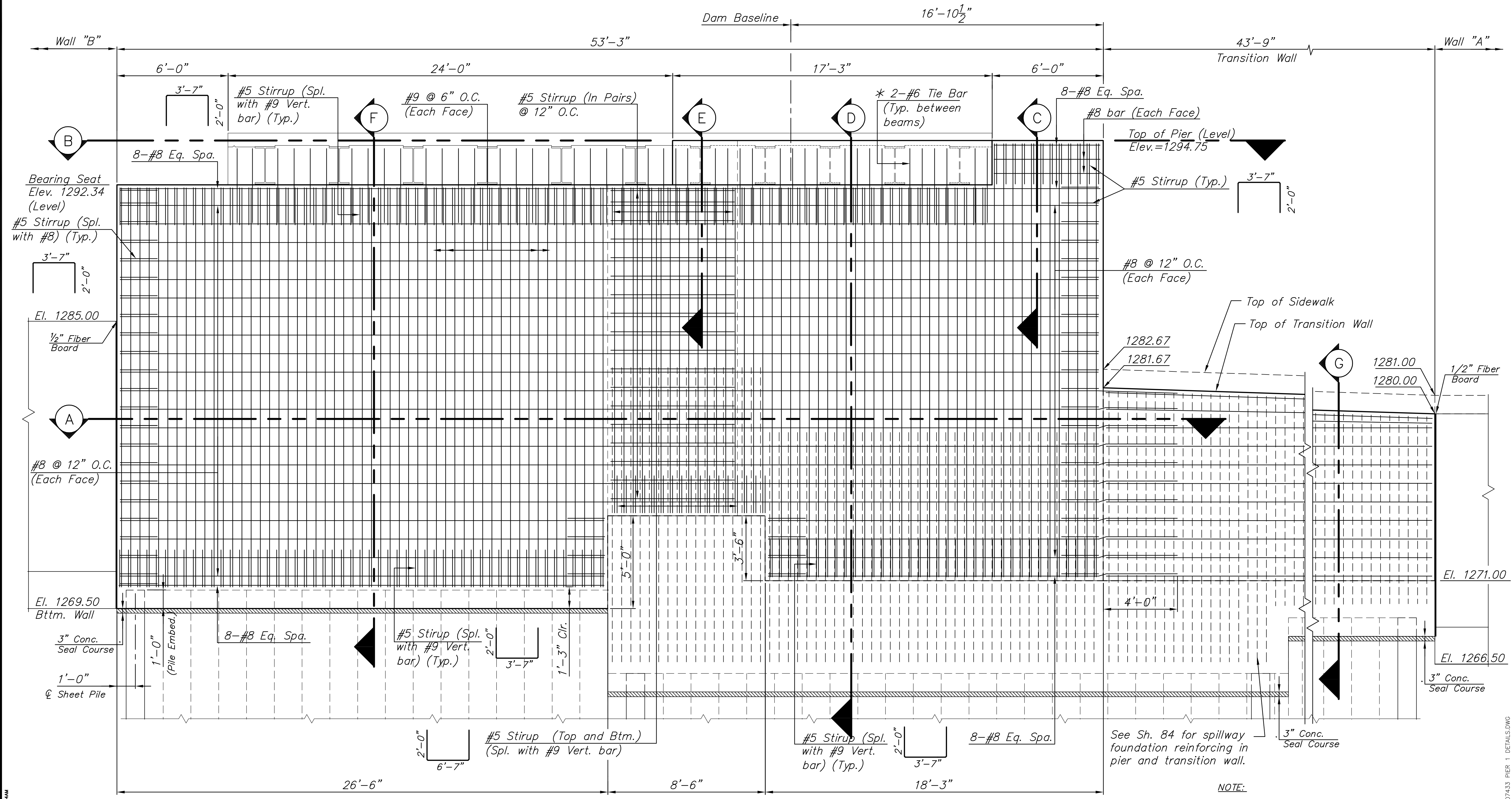
ELEVATION - PIER NO. 1 & TRANSITION WALL (Elevation Shown Looking East)
