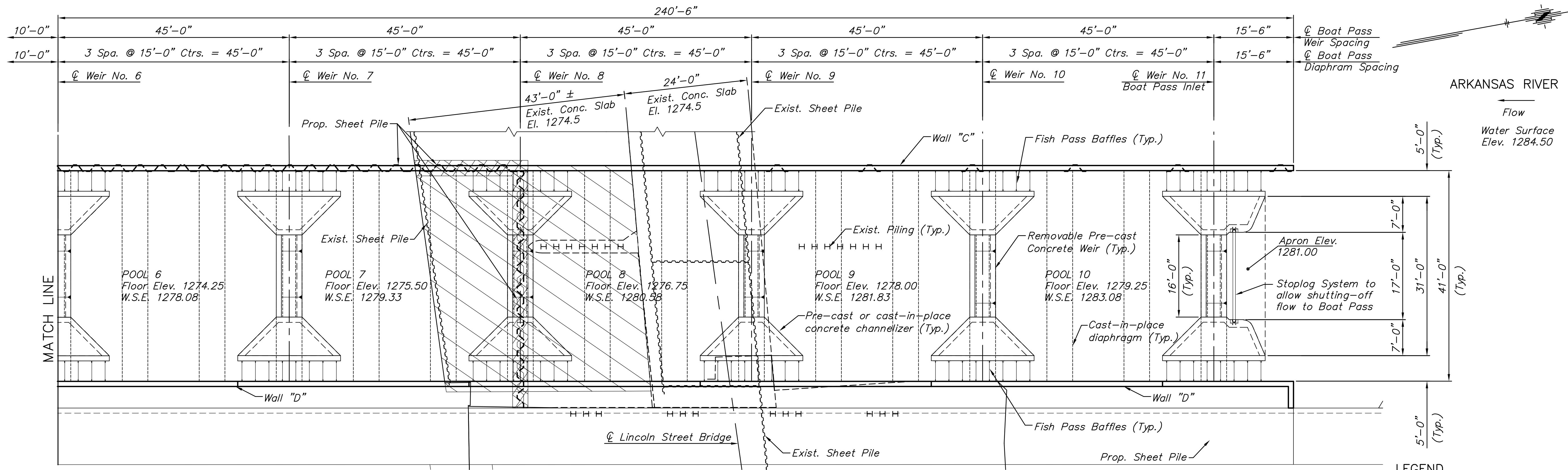
PARTIAL BOAT/FISH PASS PLAN SCALE: 3/32" = 1'-0"
