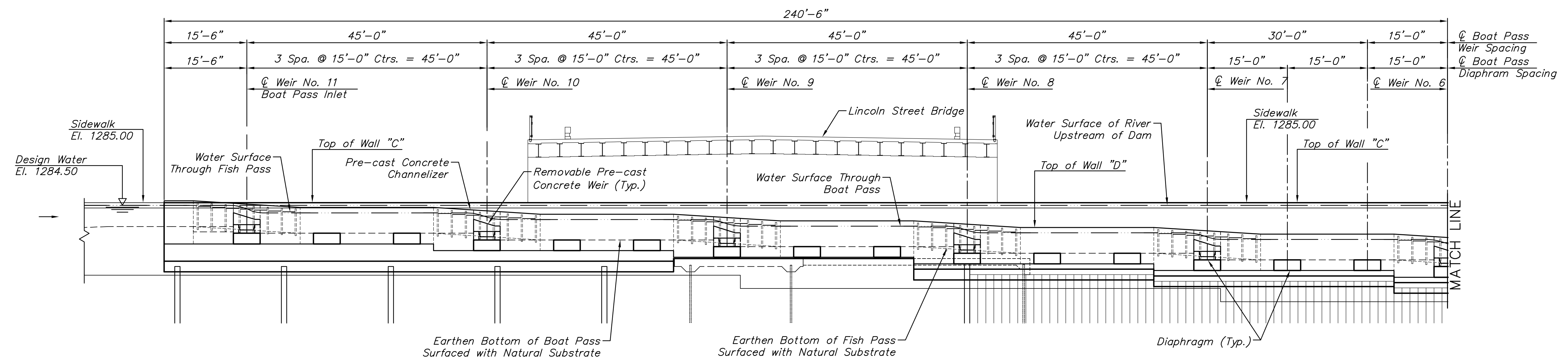
PARTIAL BOAT/FISH PASS ELEVATION SCALE: 3/32" = 1'-0"
