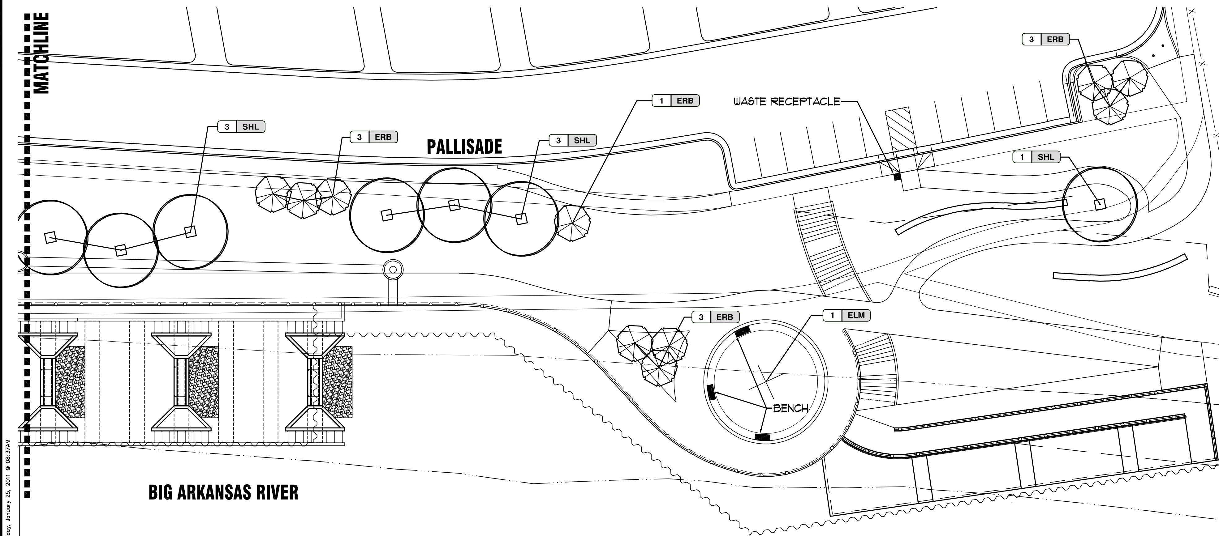
LANDSCAPE PLAN - EAST BANK
