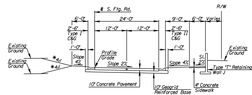
SOUTH FRONTAGE ROAD TYPICAL SECTION STA. 1685+45.82 TO STA. 1689+02.69
