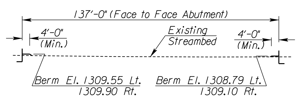
CHANNEL SECTION @ SB 143RD ST. SOUTH BRIDGE (Looking Downstream) (Along @ 143rd St.)
