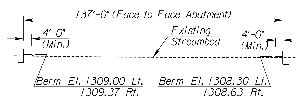
CHANNEL SECTION @ NB 143RD ST. SOUTH BRIDGE (Looking Downstream) (Along @ 143rd St.)
