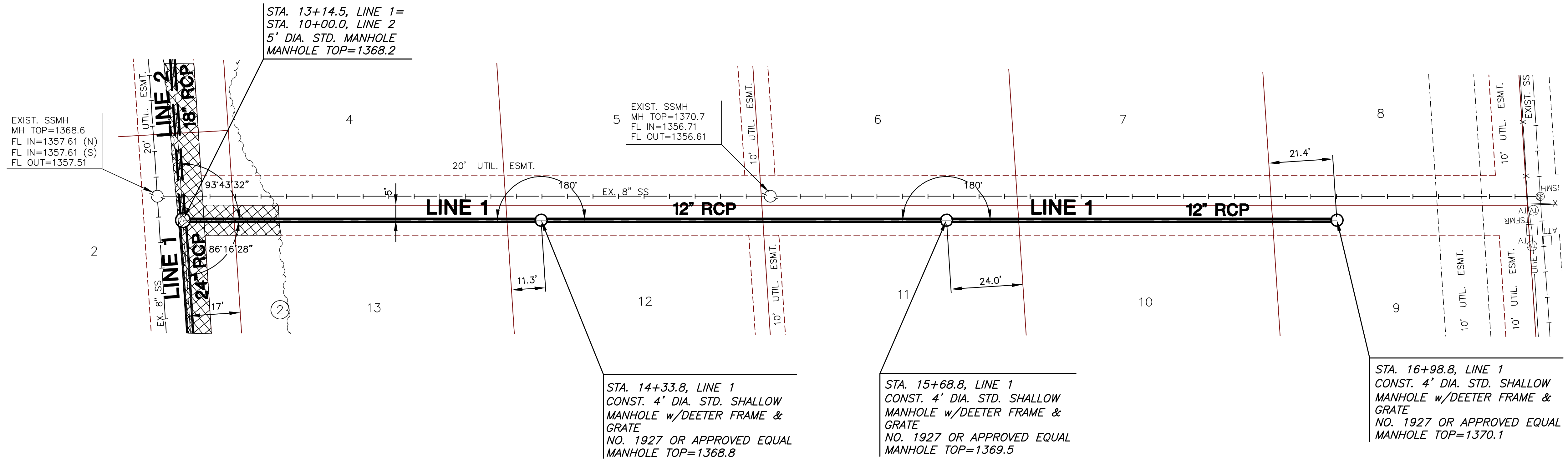
PLAN LINE 1
