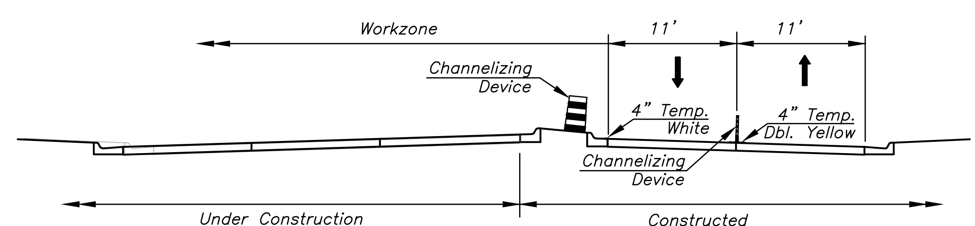
Phase 3 Traffic Control Section Looking East (31st Street South)
