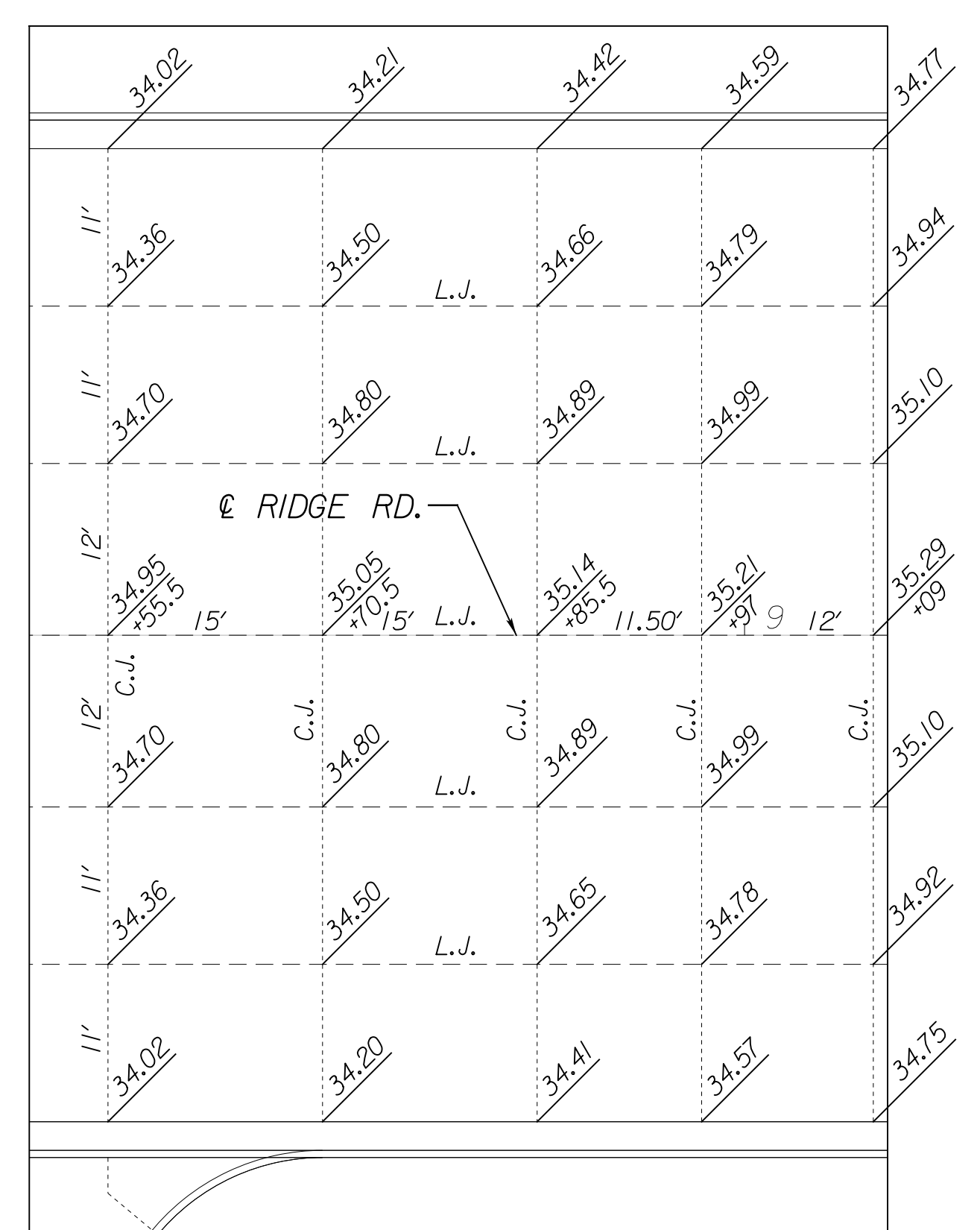
DETAIL A
