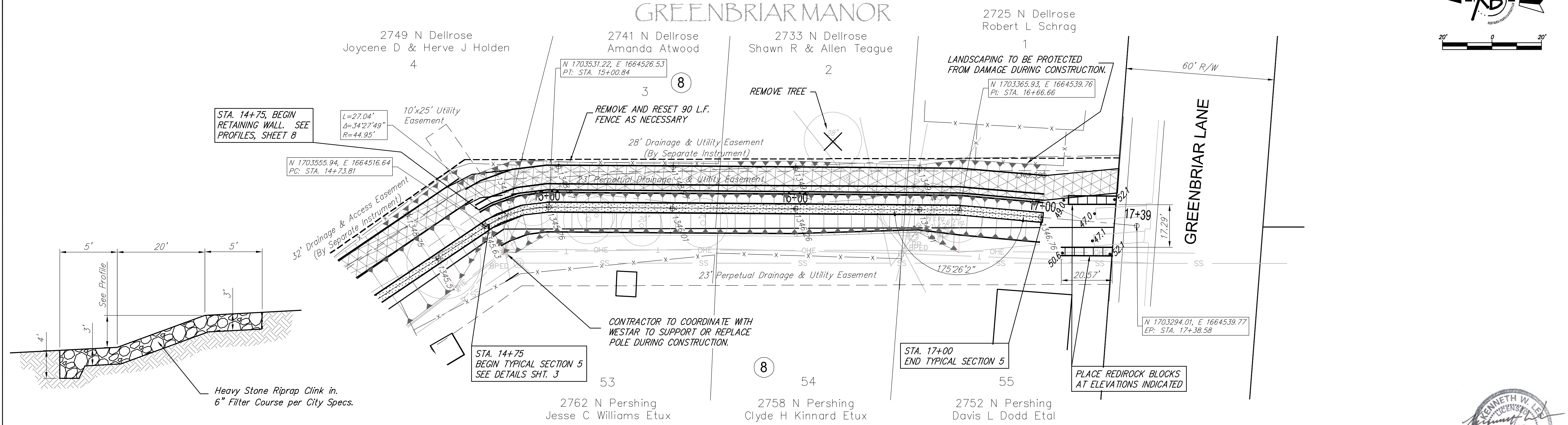
DITCH CHECK Typical 2 locations
