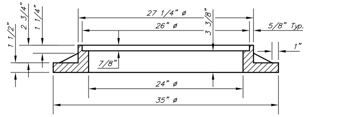
MANHOLE RING AND COVER
