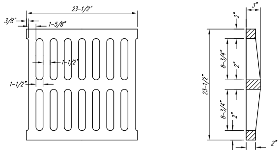
DEETER #2433 GRATE
