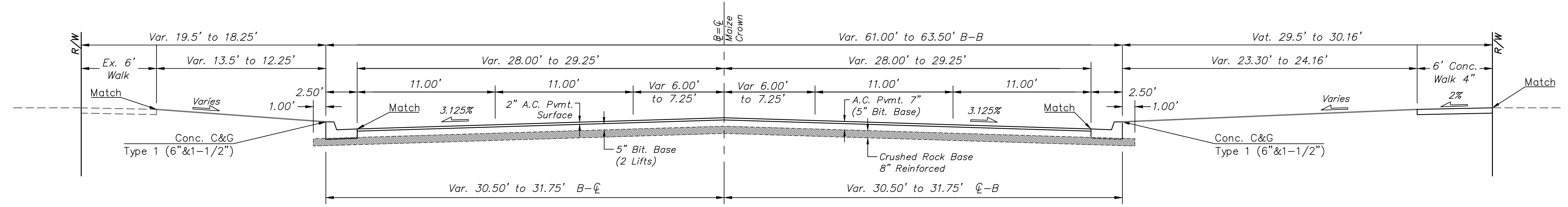
MAIZE ROAD Station 45+00.00 to Station 45+30.00
