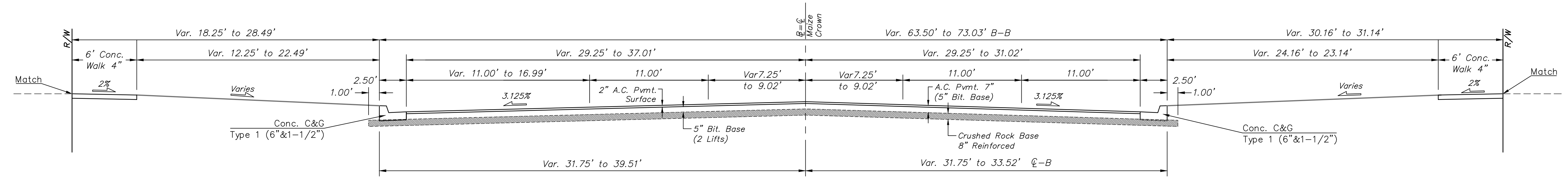
MAIZE ROAD Station 45+30.00 to Station 45+73.00
