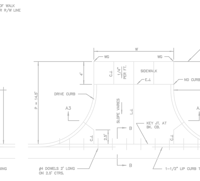
RADIUS RAMP DRIVES (P = 9.0' & GREATER)
