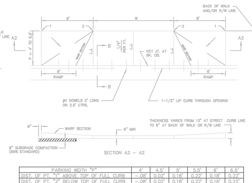
FULL RAMP DRIVE (P = 4.0' TO 6.5')
