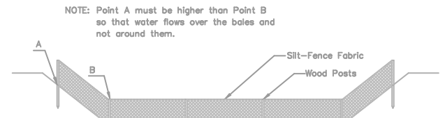
ELEVATION SILT FENCE DITCH CHECKS (STREAM PROTECTION)
