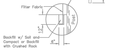
ANCHOR TRENCH DETAIL
