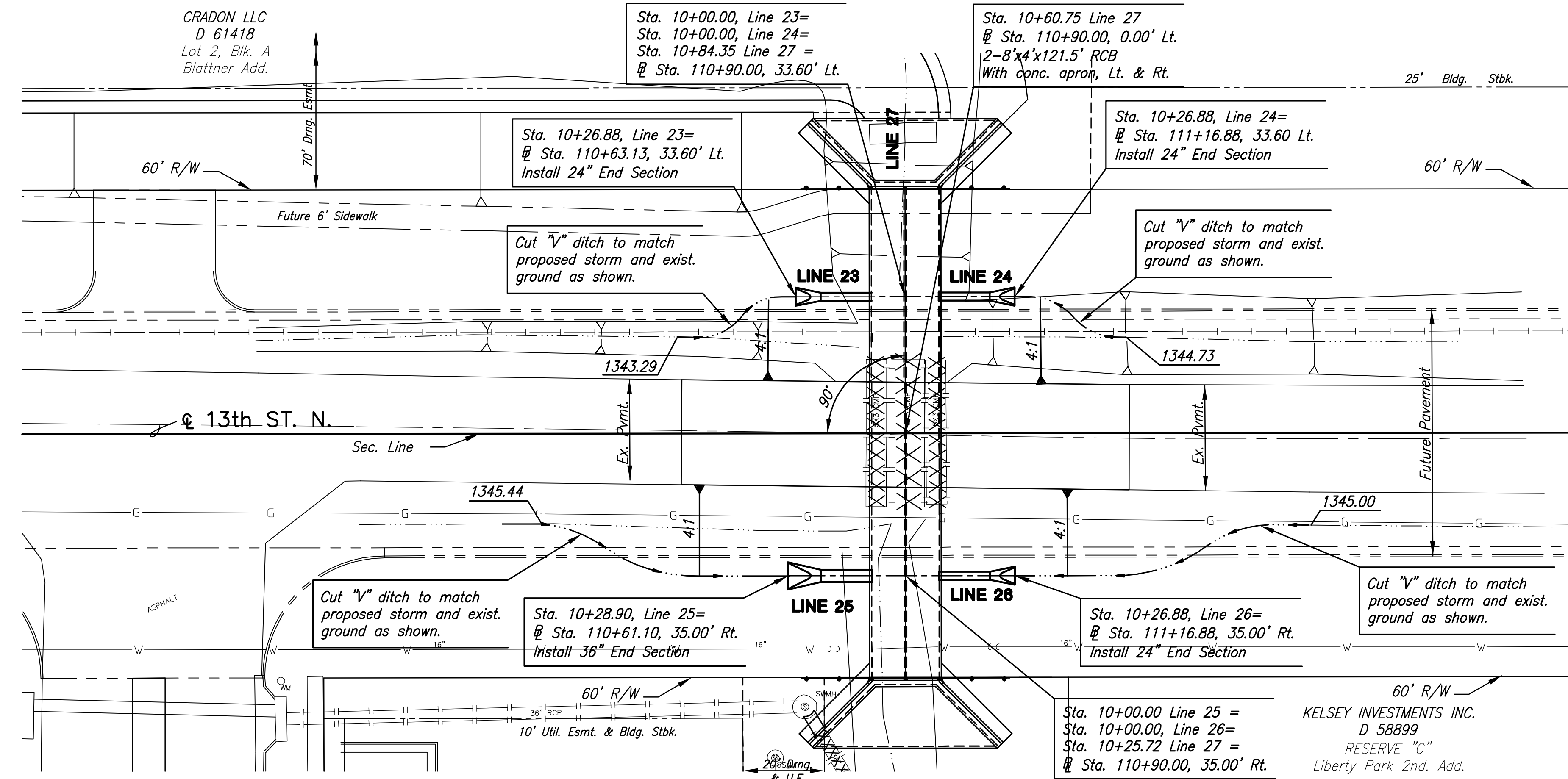
PLAN LINE 23
