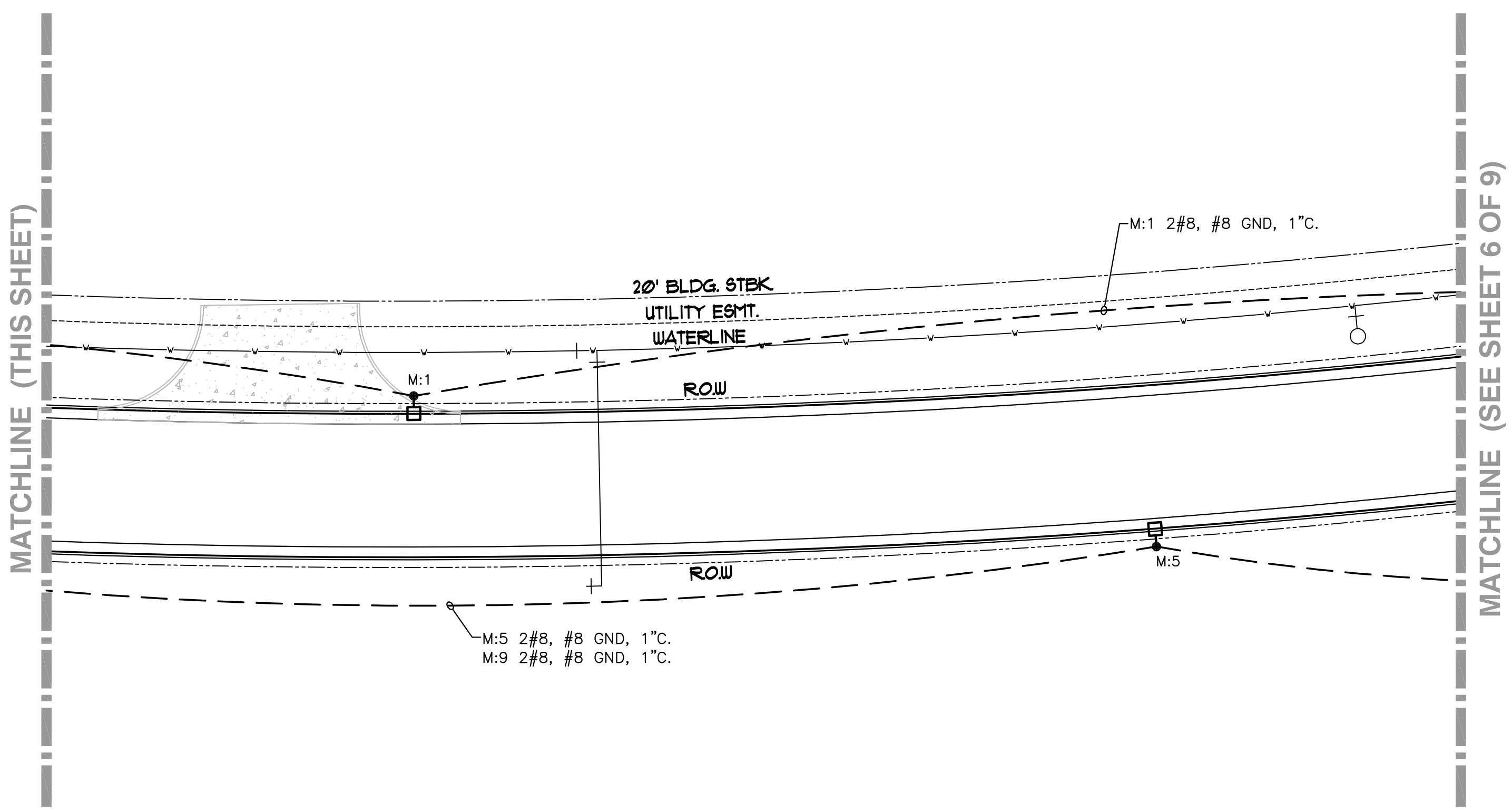
ELECTRICAL PLAN SCALE: 1" = 20'-0" SCALE 1" = 20'-0"
