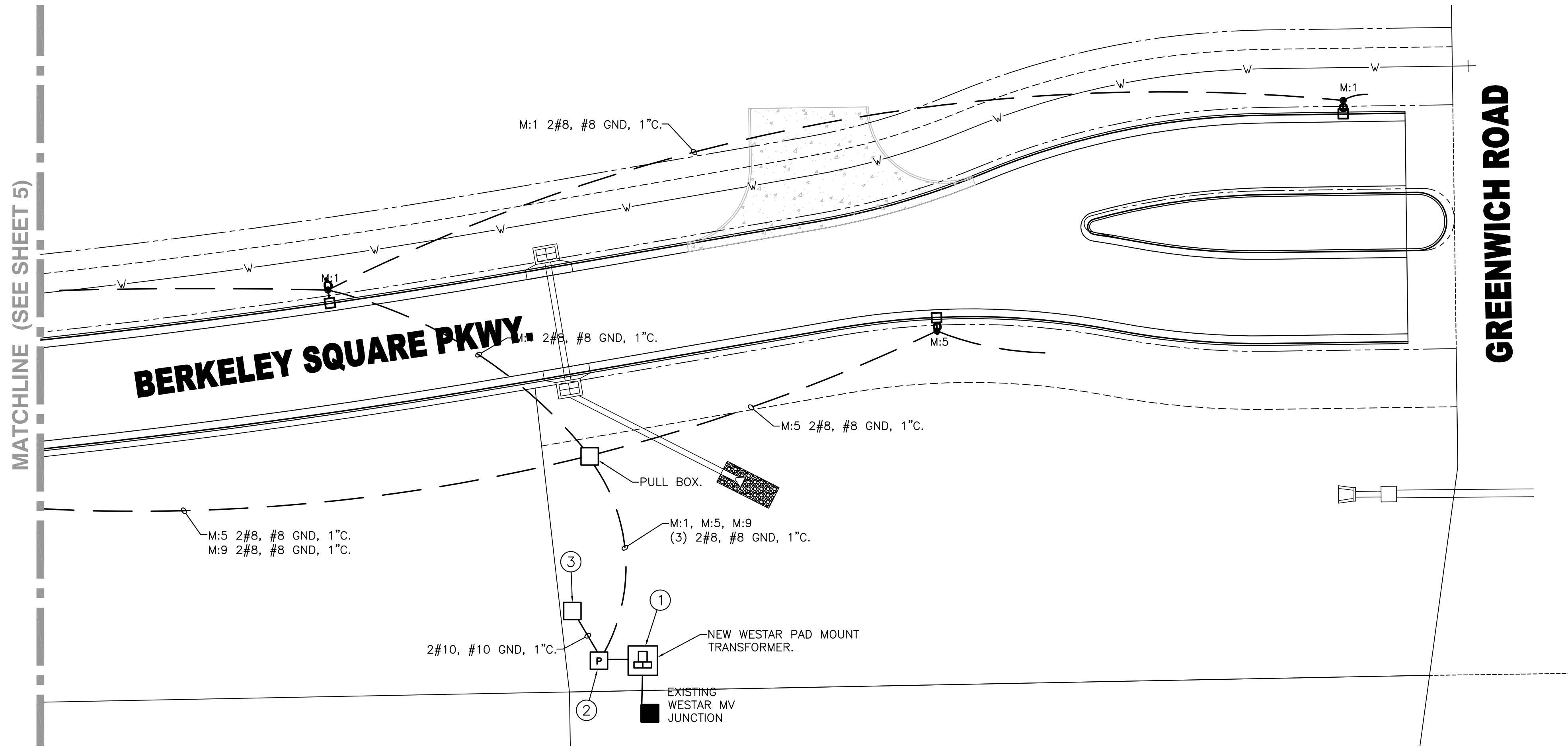
ELECTRICAL PLAN SCALE: 1" = 20'-0"
