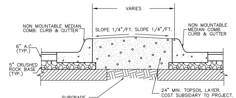
MEDIAN DETAIL SCALE: NONE
