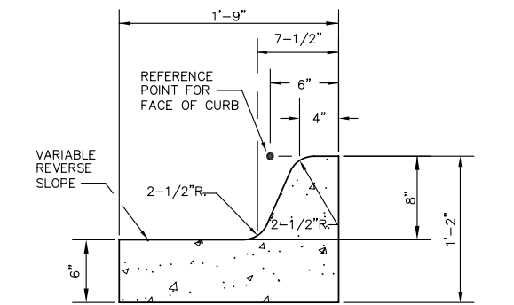
NON MOUNTABLE MEDIAN COMBINED CURB & GUTTER (8") SCALE: NONE
