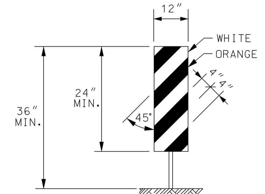
VERTICAL PANEL
