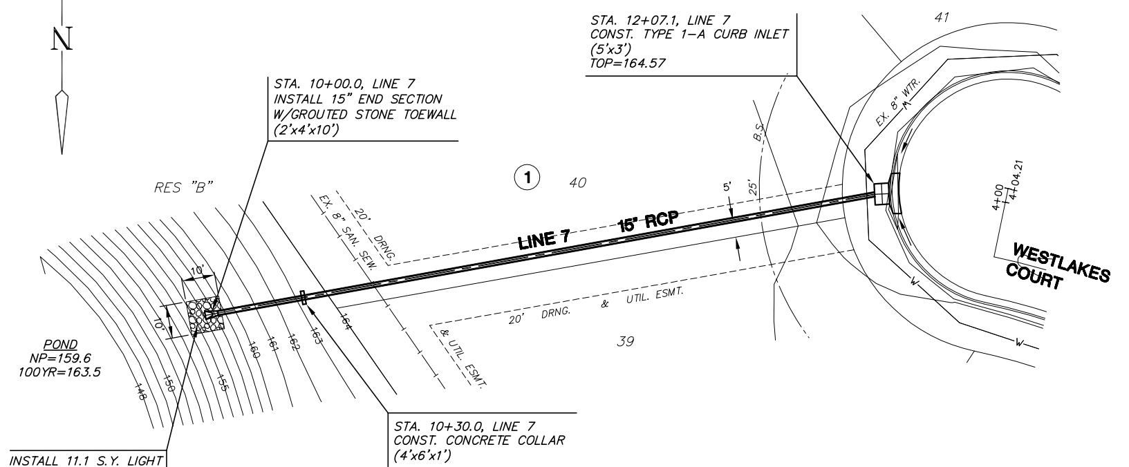
PLAN LINE 7
