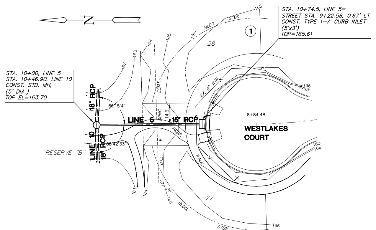
PLAN LINE 5
