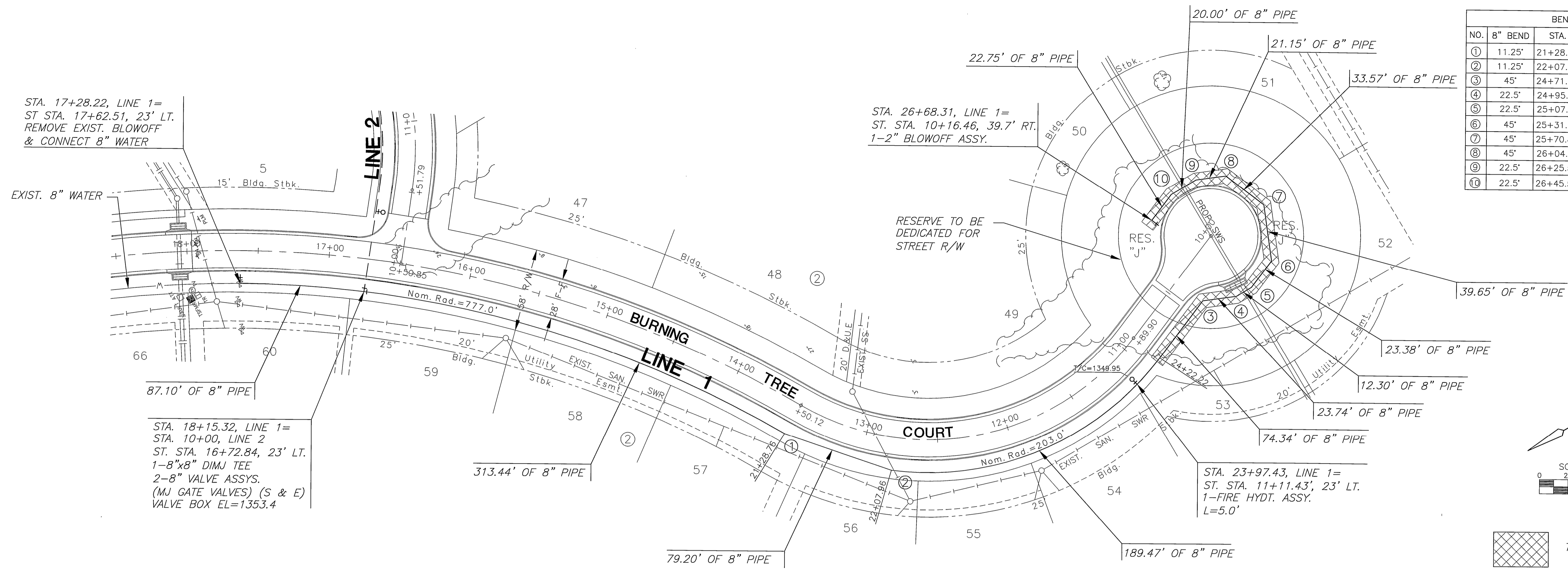
PLAN LINE 1
