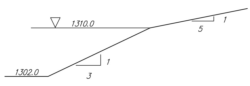
POND GRADING SECTION
