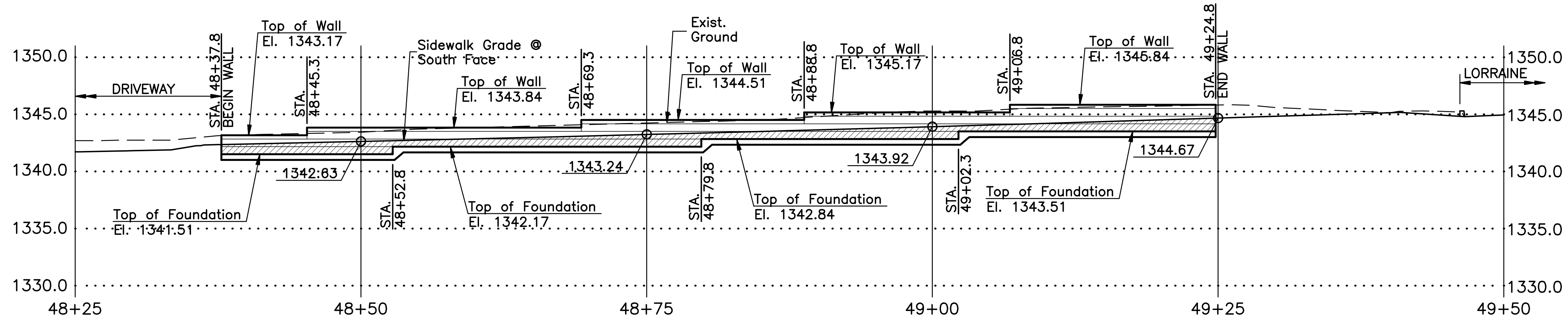
MODULAR CONC. RETAINING WALL PROFILE 13th Street Sta. 48+37.8 to Sta. 49+24.8 Lt.
