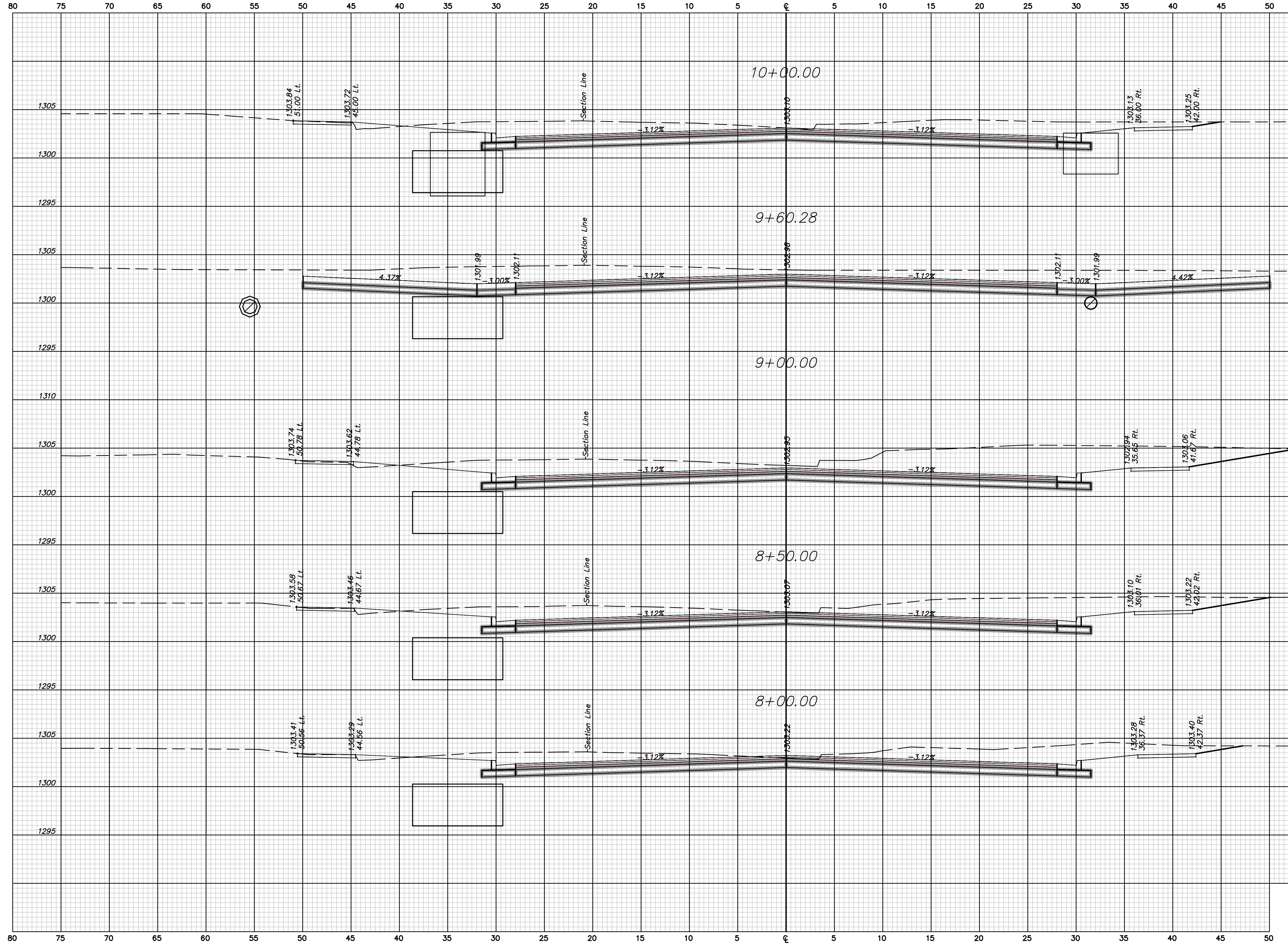
13th STREET CROSS SECTIONS Sta. 8+00.00 to Sta. 10+00.00
