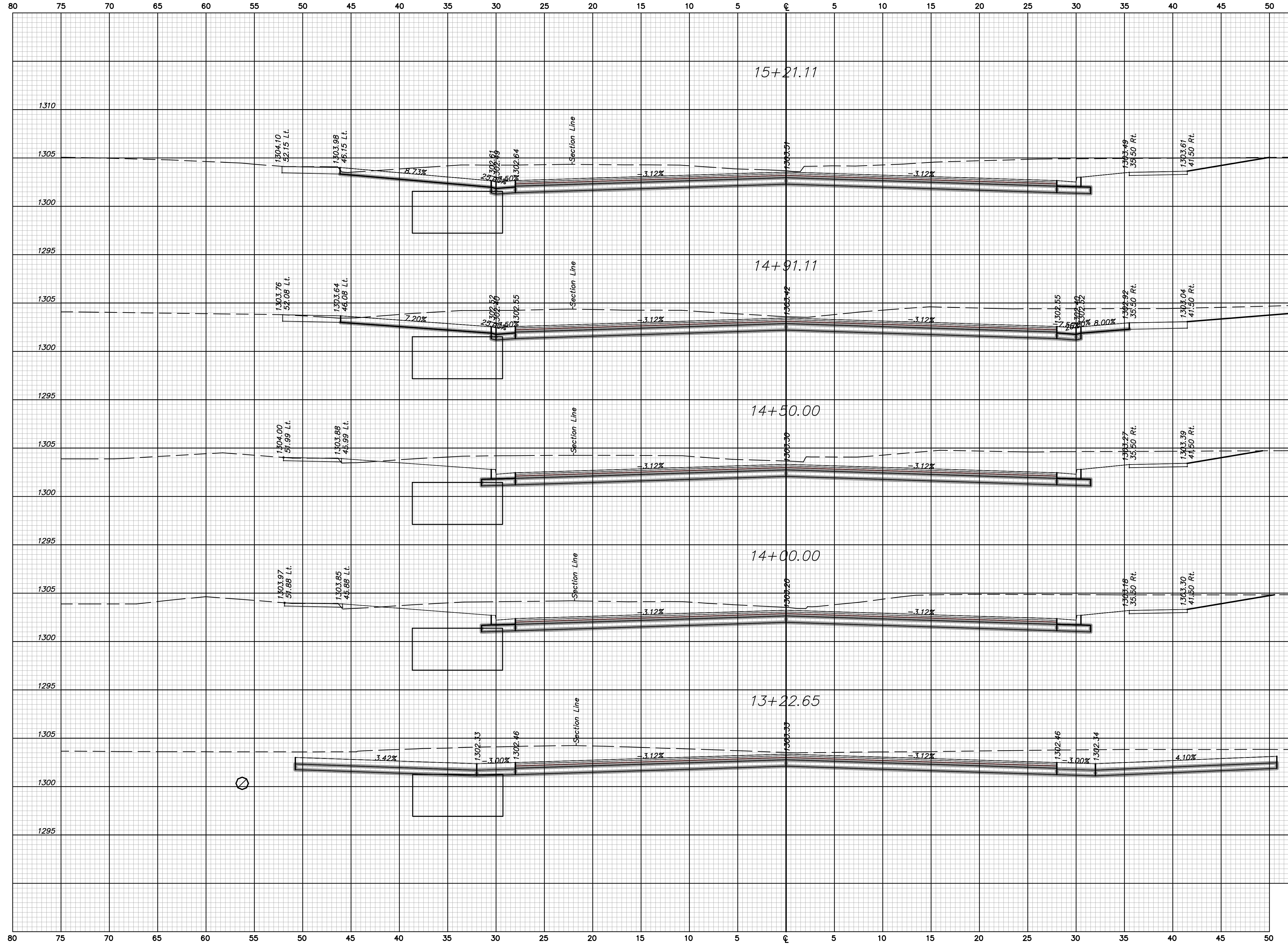
13th STREET CROSS SECTIONS Sta. 13+22.65 to Sta. 15+21.11
