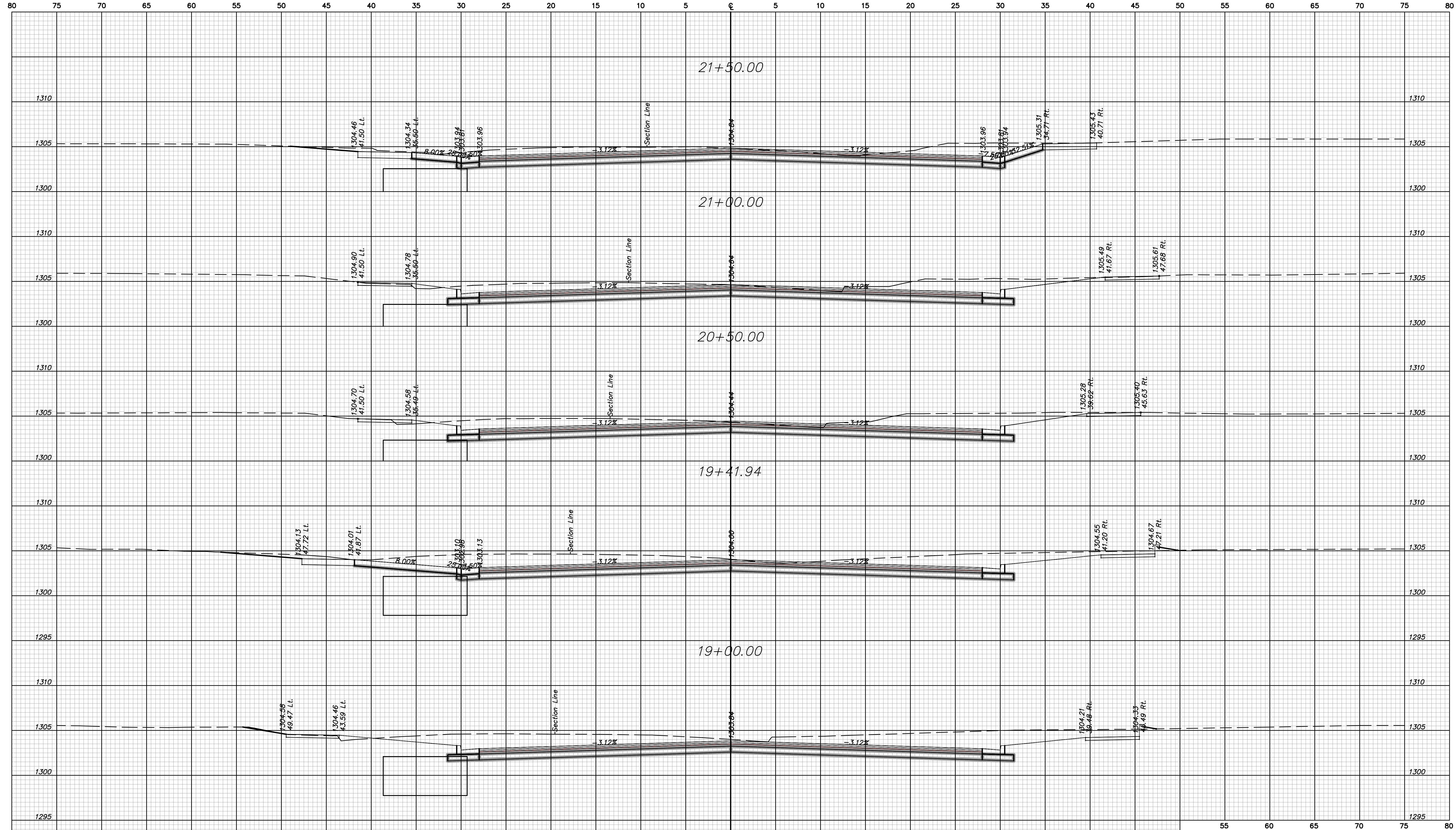
13th STREET CROSS SECTIONS Sta. 19+00.00 to Sta. 21+50.00
