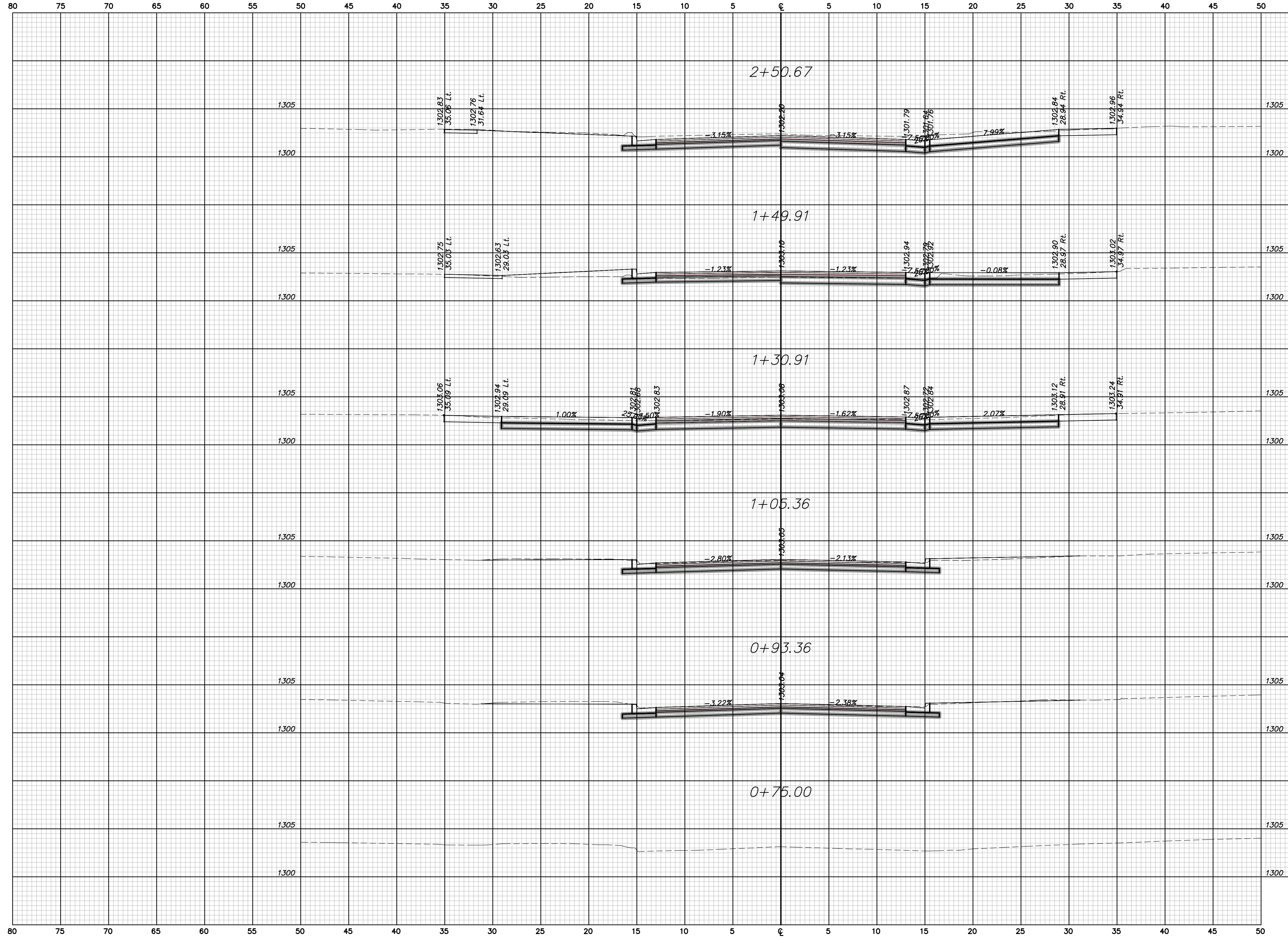
KANSAS AVENUE CROSS SECTIONS Sta. 0+75.00 to Sta. 2+50.67
