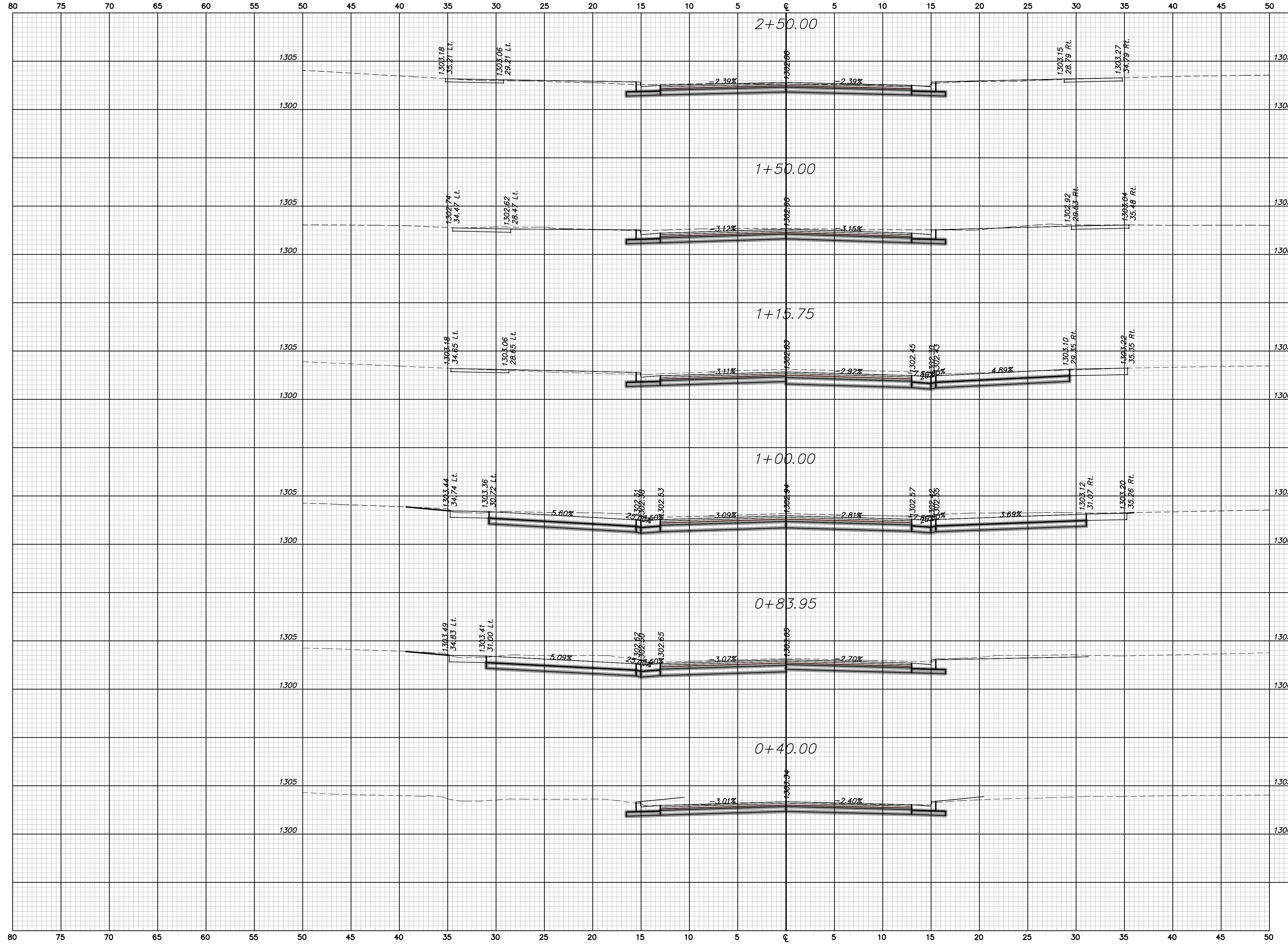
MINNEAPOLIS AVENUE CROSS SECTIONS Sta. 0+40.00 to Sta. 2+50.00
