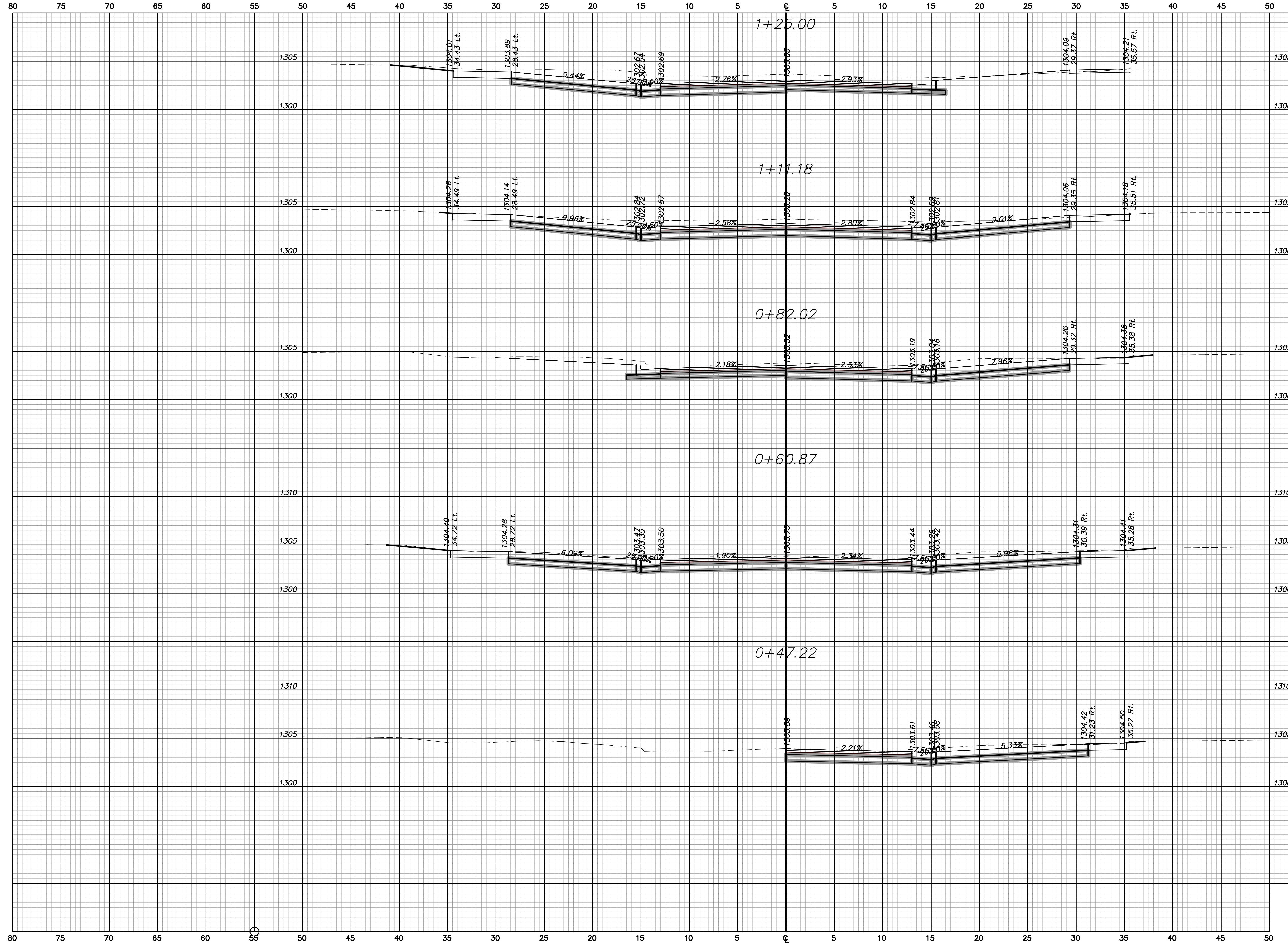
MINNESOTA AVENUE CROSS SECTIONS Sta. 0+50.00 to Sta. 1+50.00
