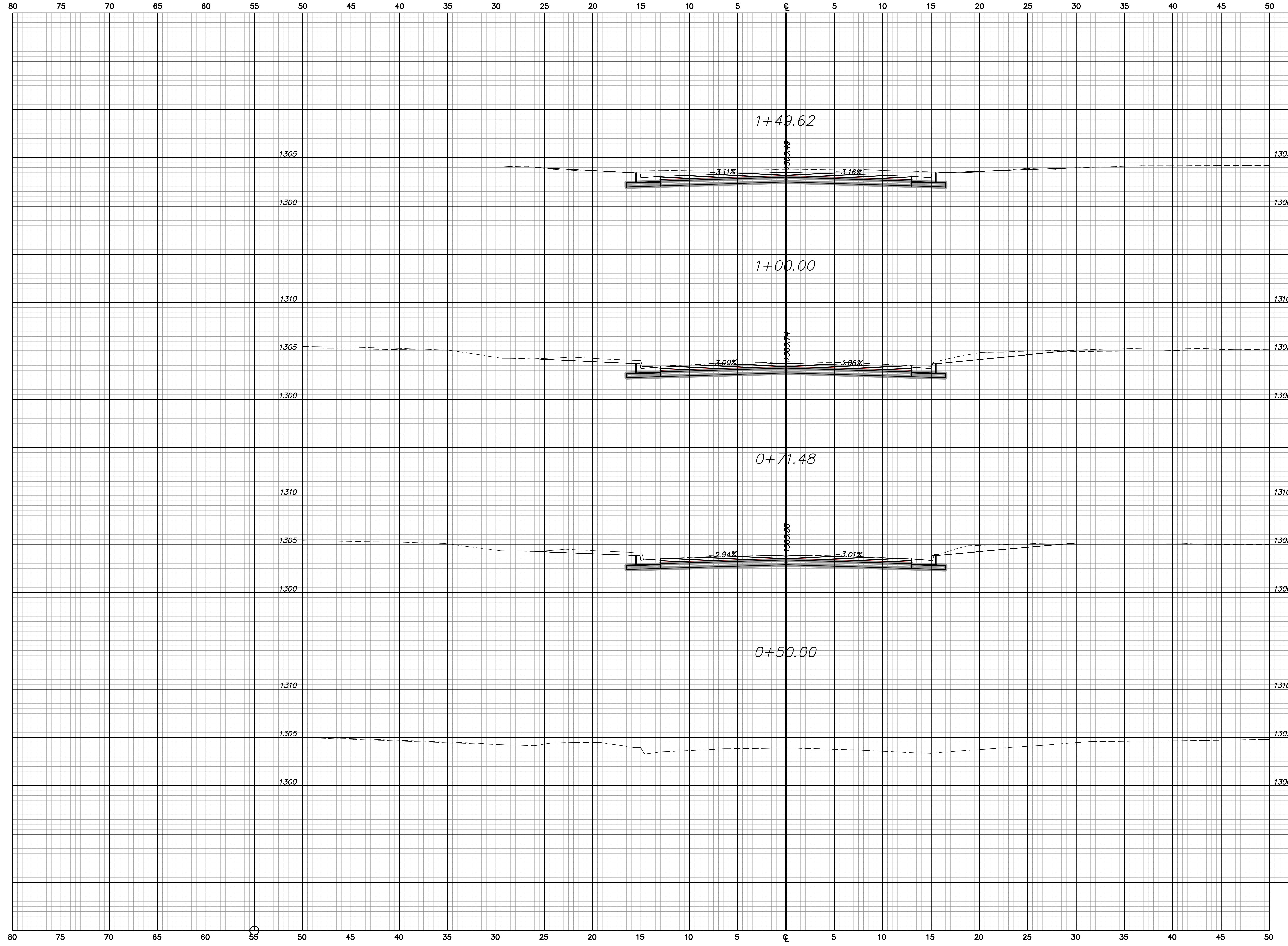
ASH CROSS SECTIONS Sta. 0+50.00 to Sta. 1+49.62
