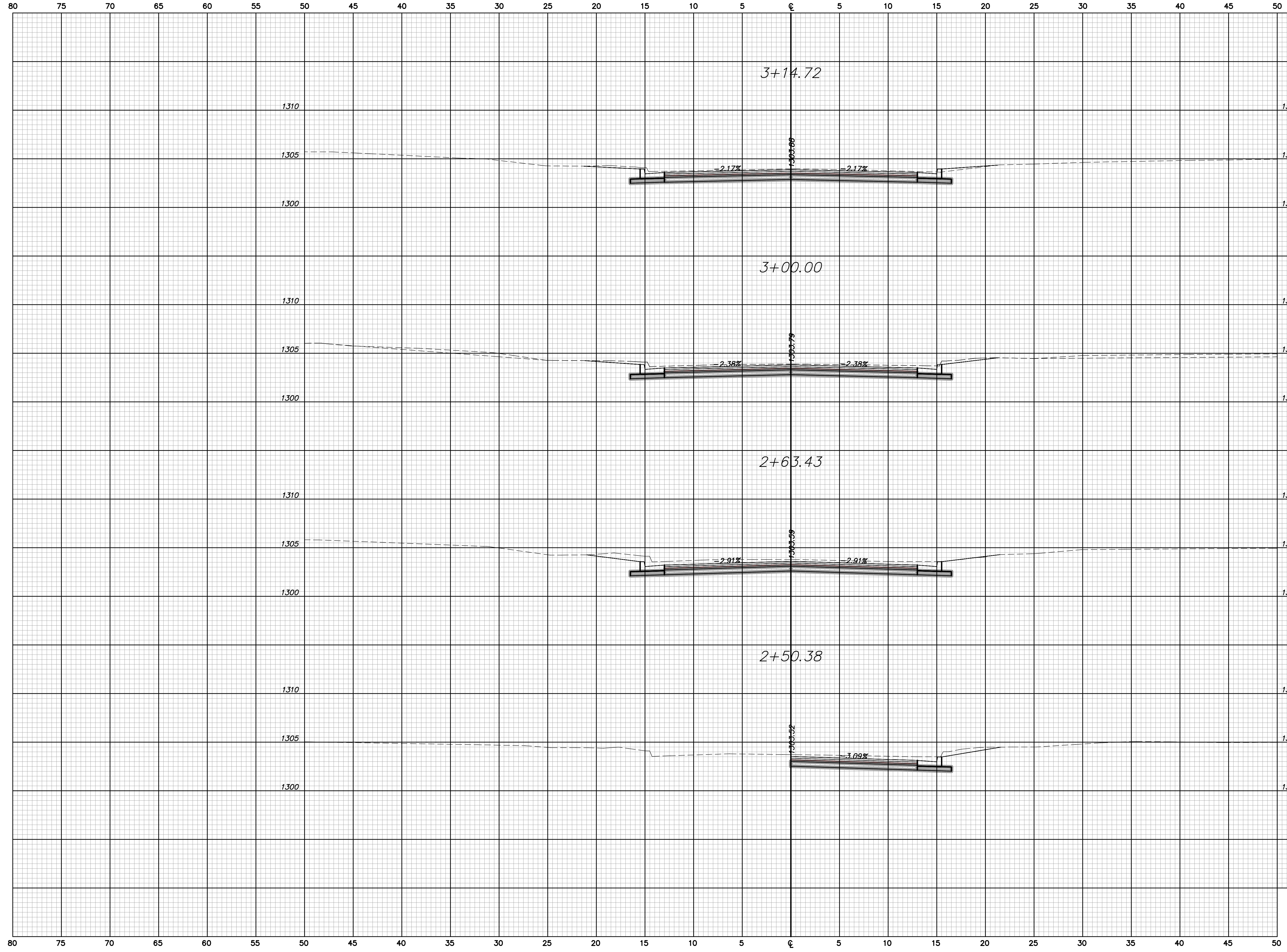
ASH CROSS SECTIONS Sta. 2+50.38 to Sta. 3+14.72
