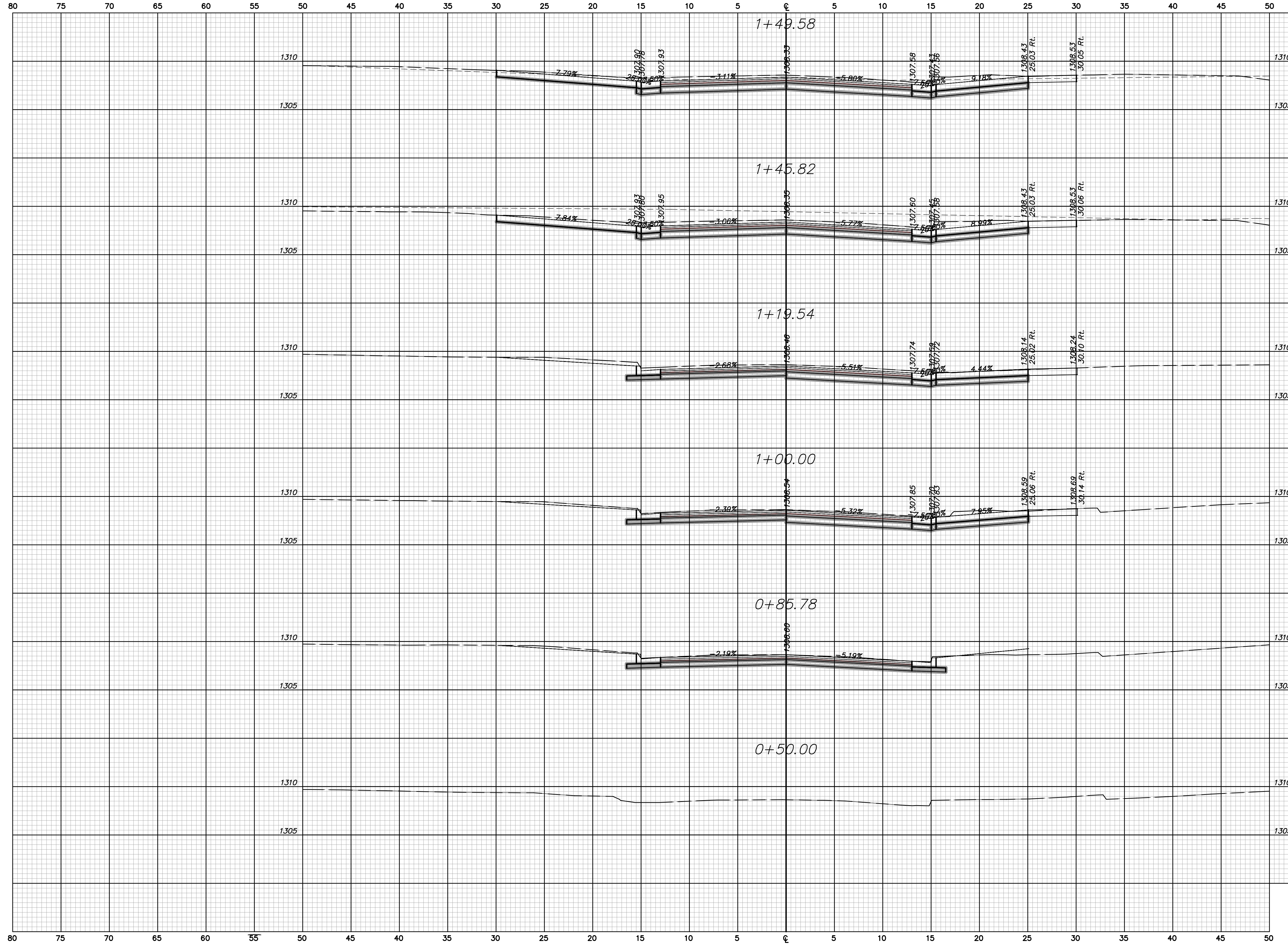
POPLAR CROSS SECTIONS Sta. 0+50.00 to Sta. 1+49.58
