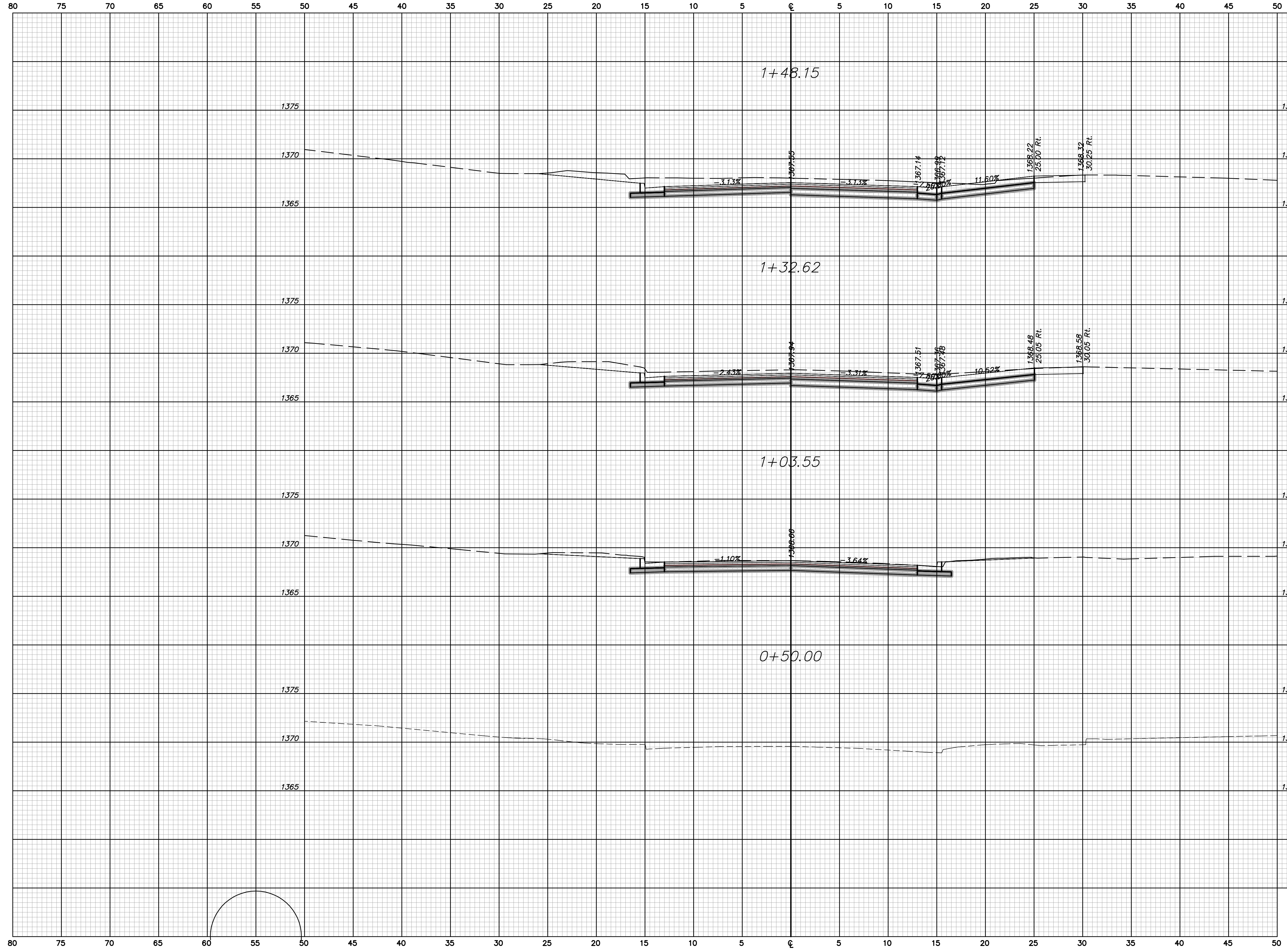
HOLYOKE CROSS SECTIONS Sta. 0+50.00 to Sta. 1+48.15
