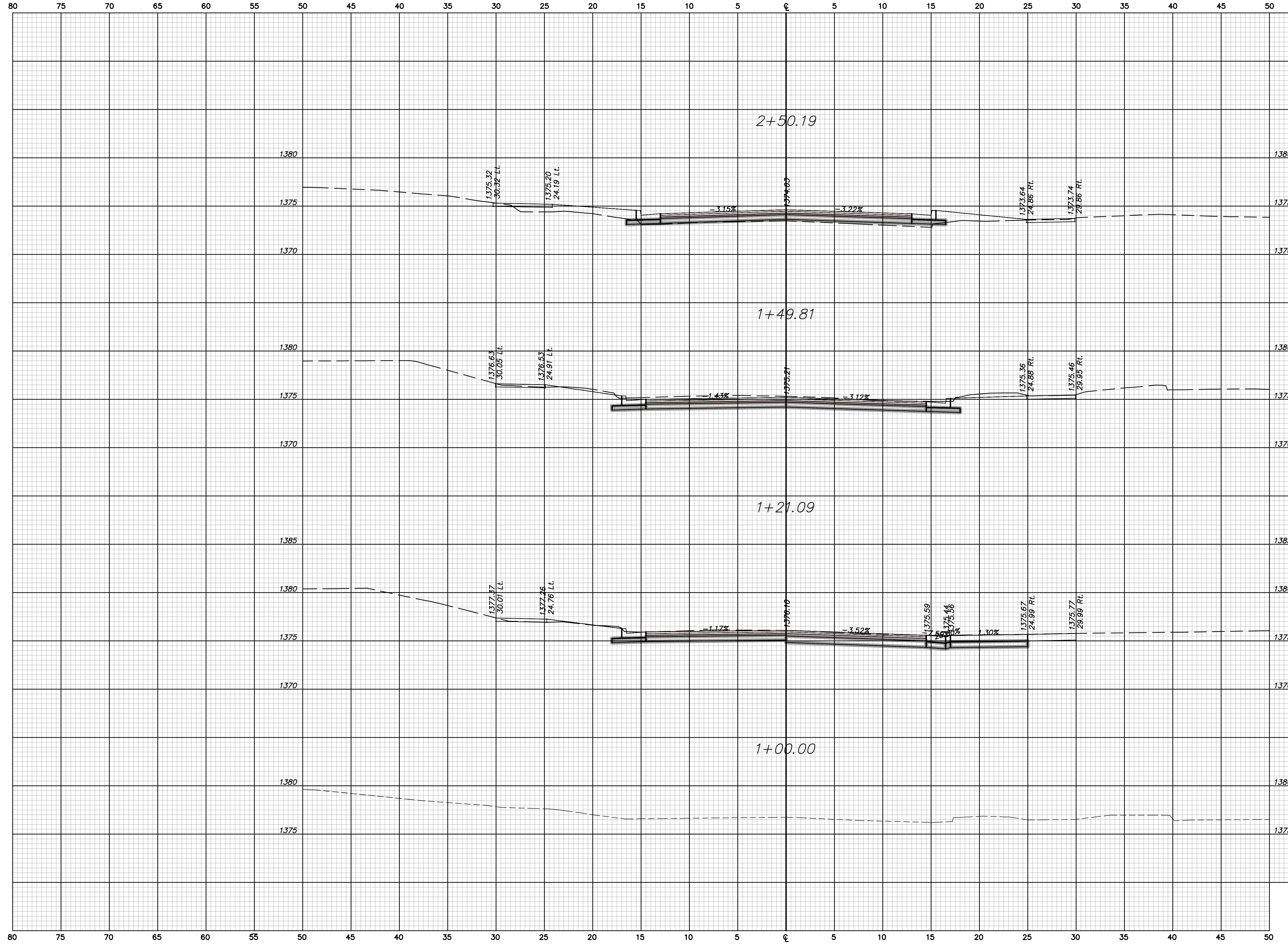
FAIRMOUNT CROSS SECTIONS Sta. 1+00.00 to Sta. 2+50.19
