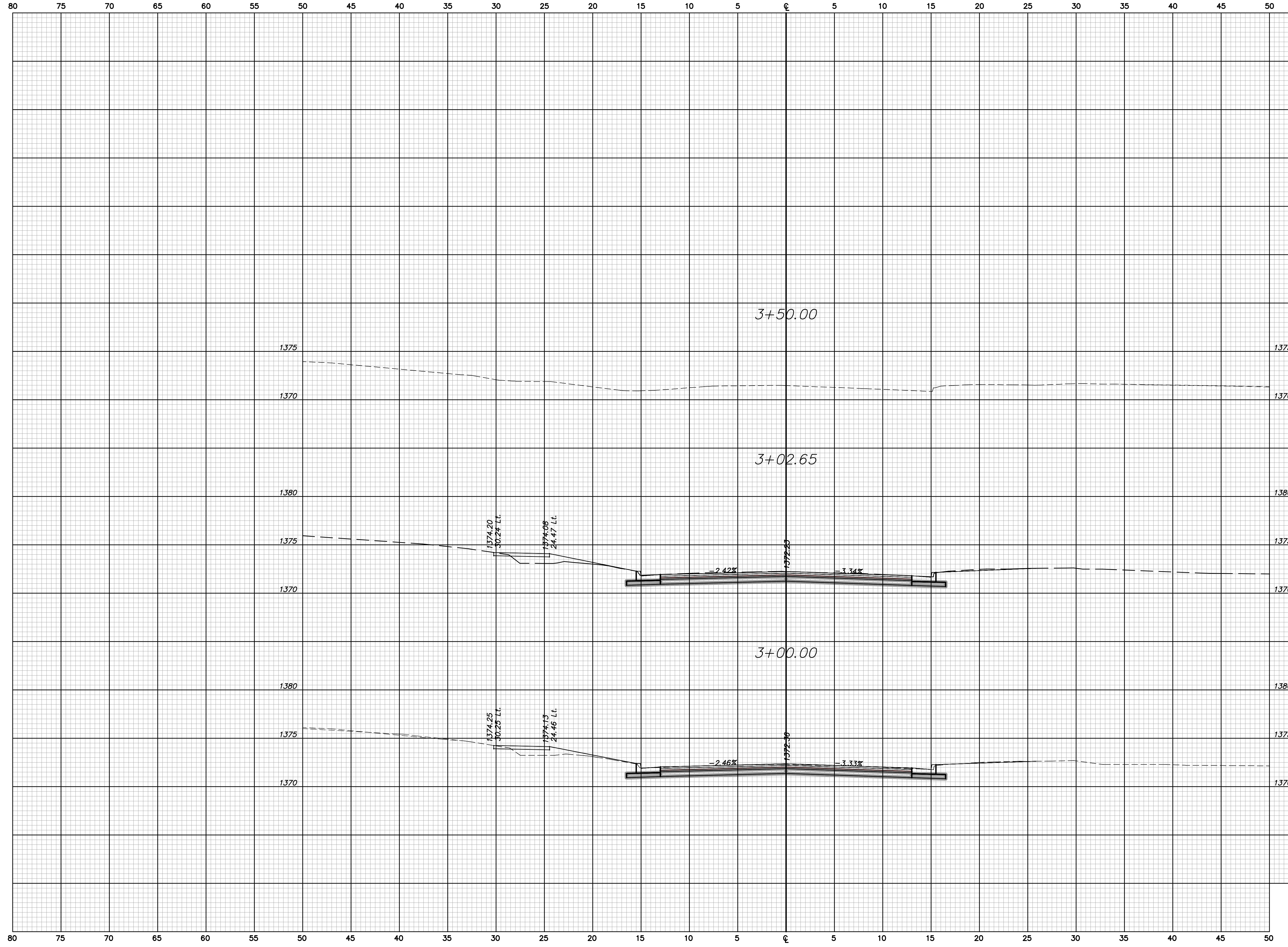
FAIRMOUNT CROSS SECTIONS Sta. 3+00.00 to Sta. 3+50.00
