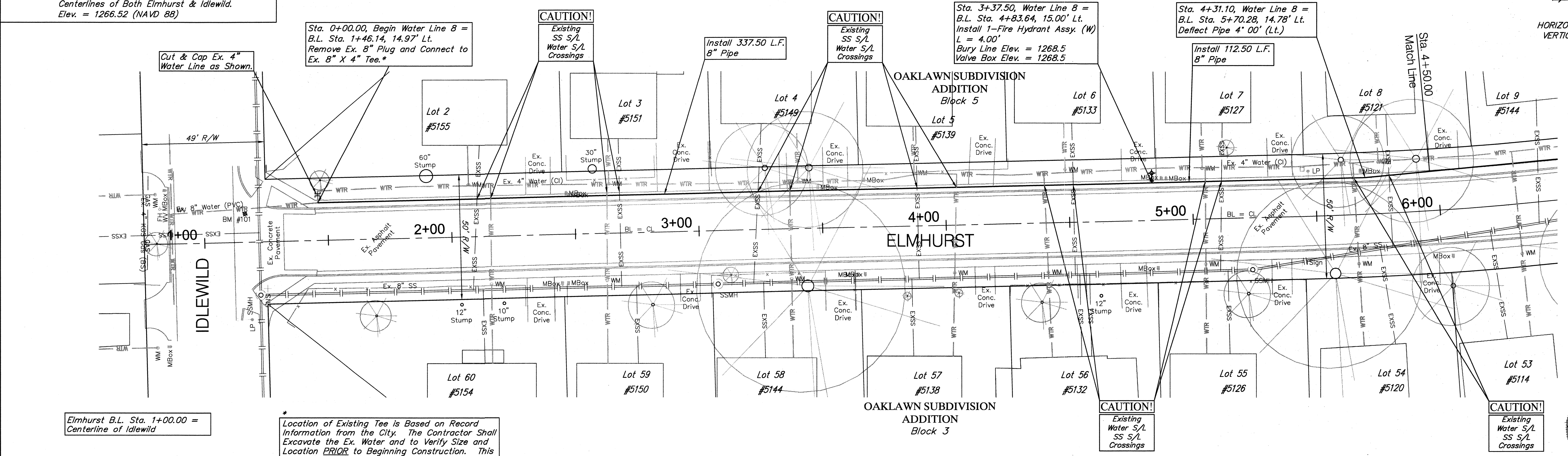
Water Line 8
