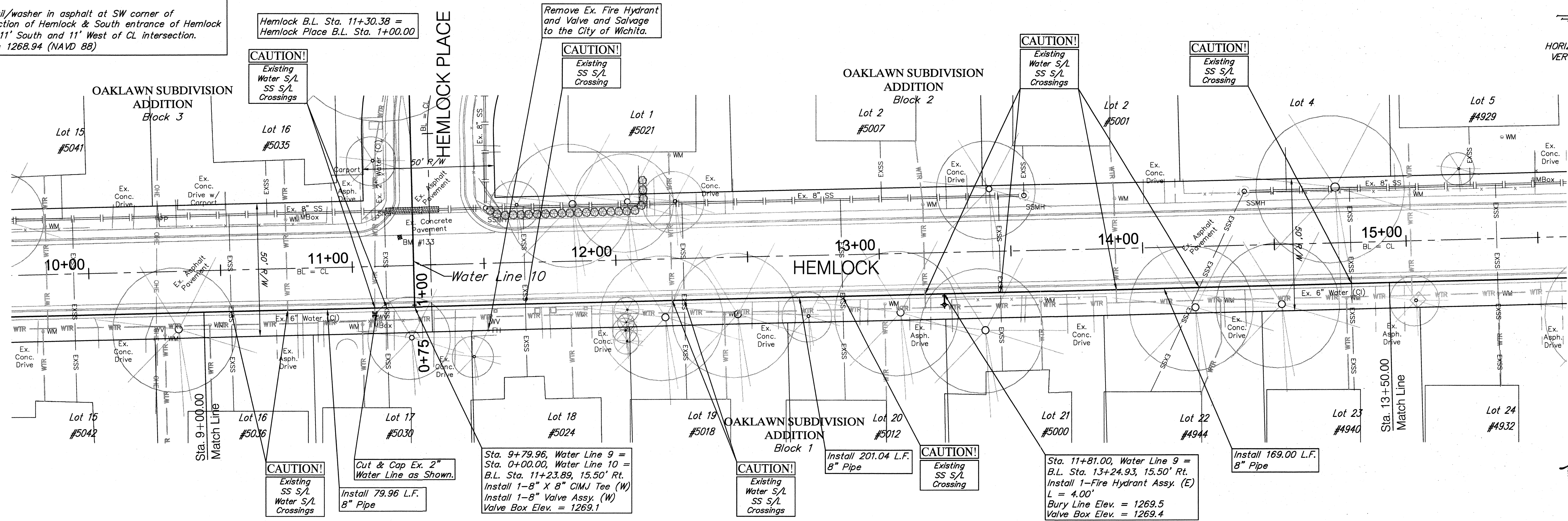
Water Line 9
